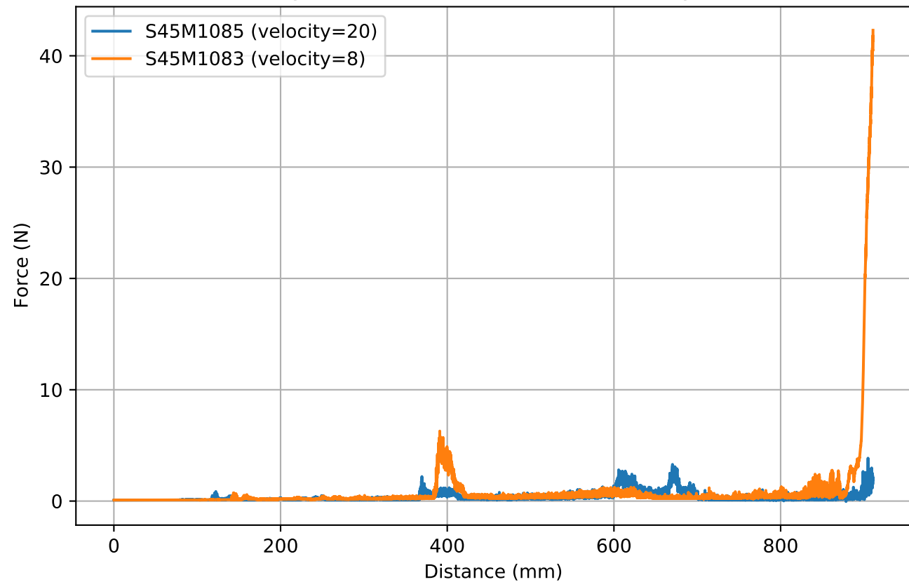
Aligned: S45M1085 to S45M1083 (Day 2)
