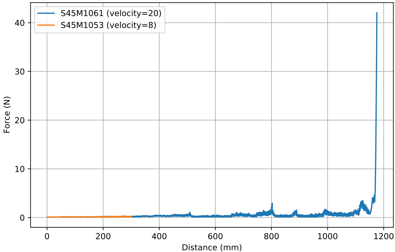
Aligned: S45M1061 to S45M1053
