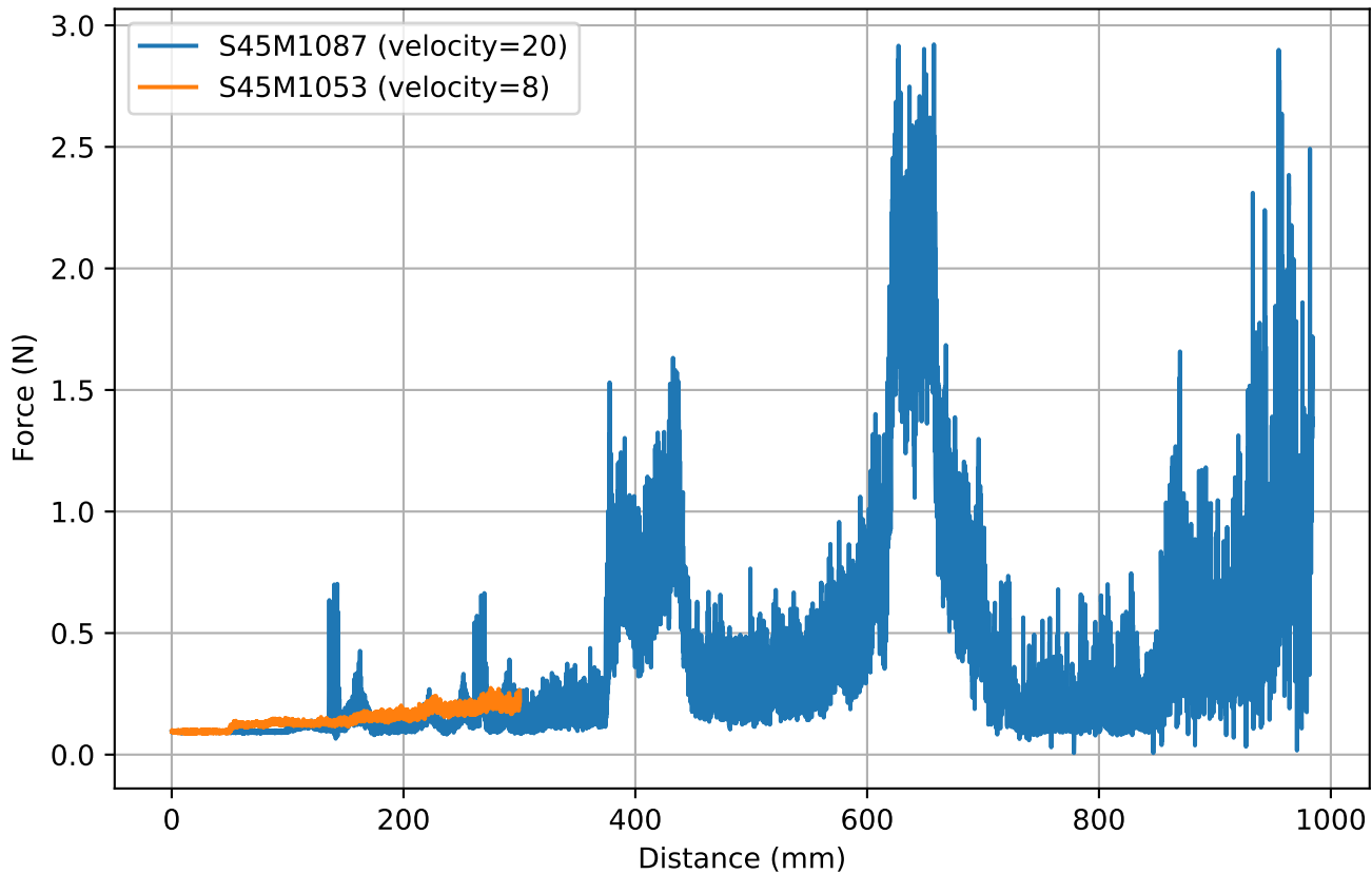
Aligned: S45M1087 to S45M1053
