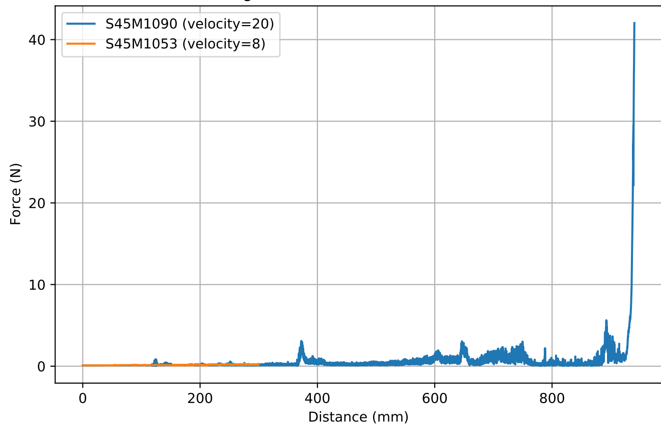
Aligned: S45M1090 to S45M1053
