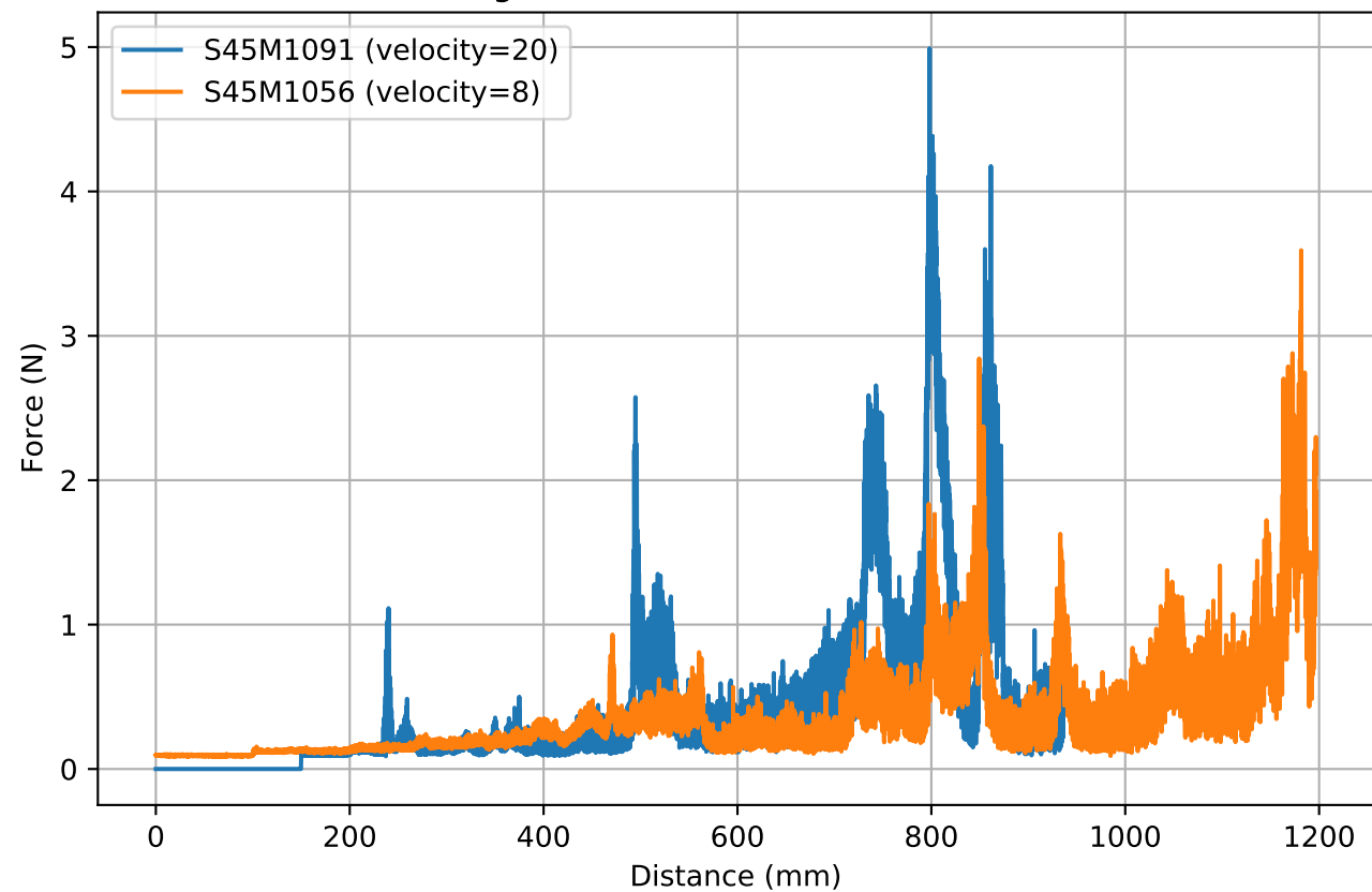
Aligned: S45M1091 to S45M1056
