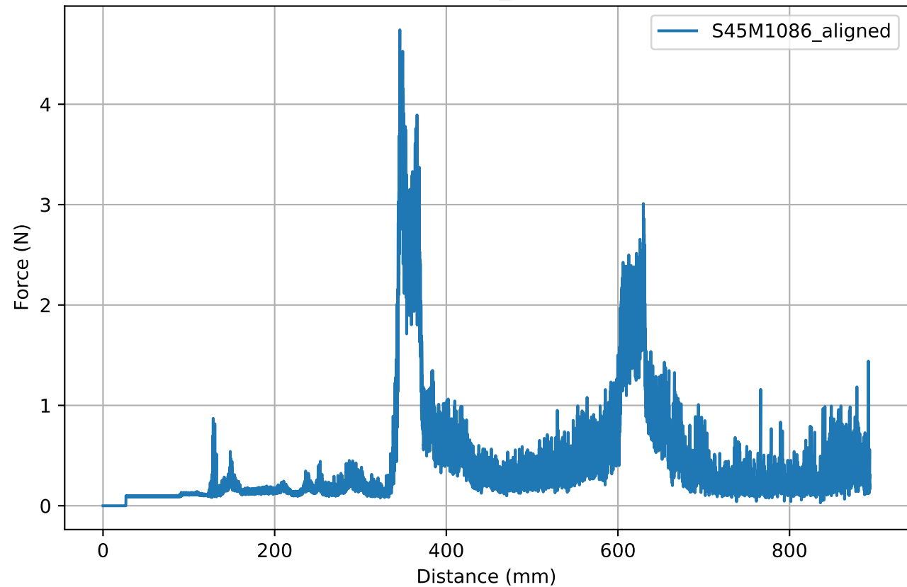
S45M1086_aligned
