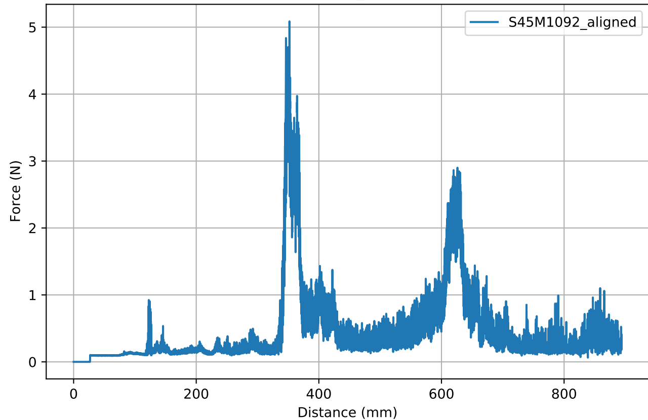
S45M1092_aligned
