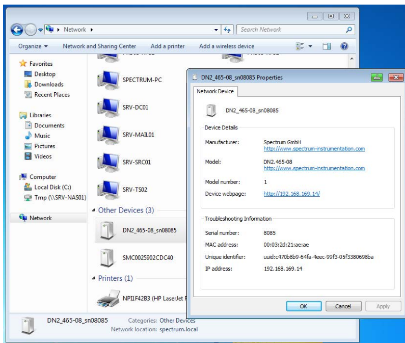
Image 94: Windows screenshot: finding a remote Spectrum device like digitizerNETBOX
