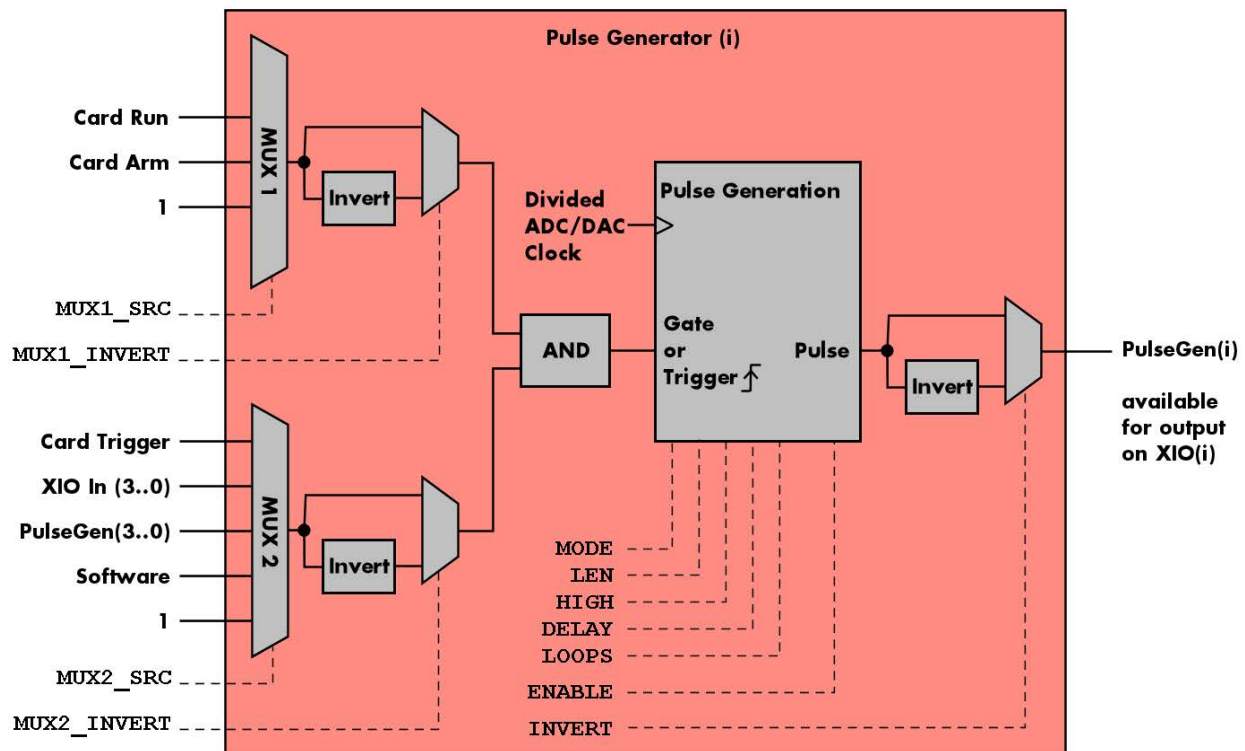
Image 86: overview block diagram of the pulse generator
