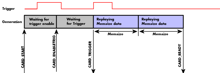
Image 53: timing diagram of single replay mode with two loops with commands and status changes
