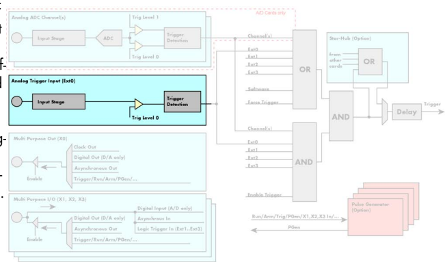
Image 65: trigger engine overview and external trigger
