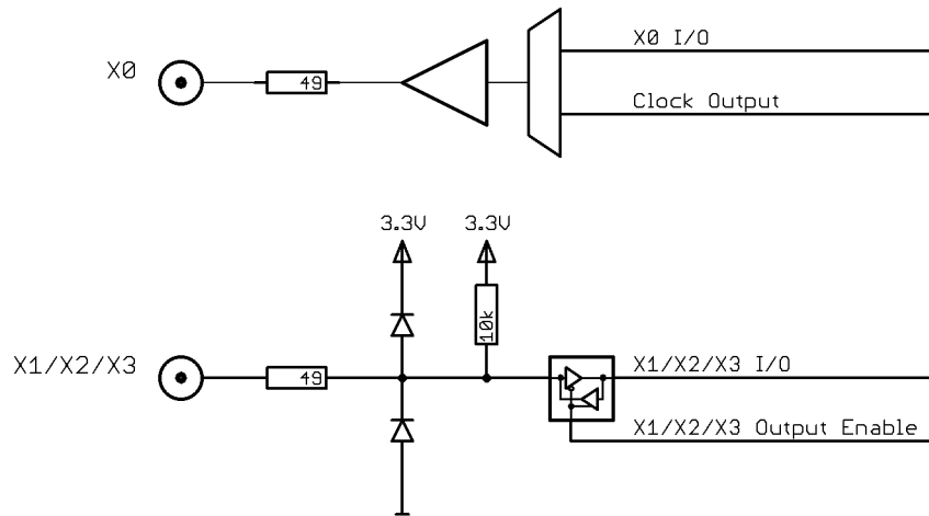
Image 99: electrical connection and termination of multi-purpose I/O lines
