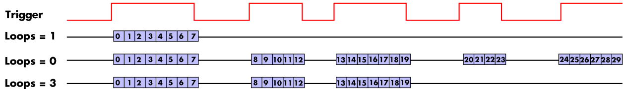
Image 75: timing diagram of Gated Replay FIFO mode depending on different loops settings
