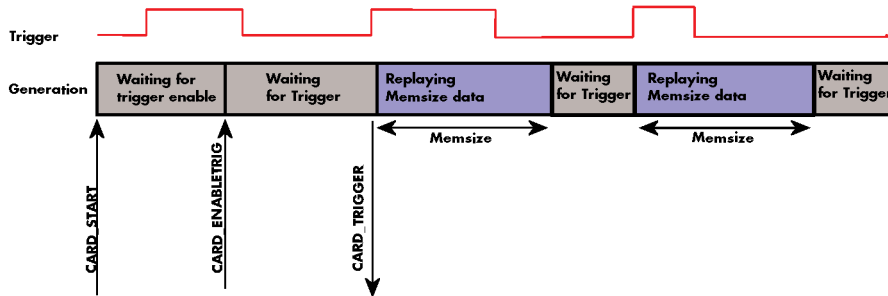
Image 55: timing diagram of single restart mode with commands and status changes
