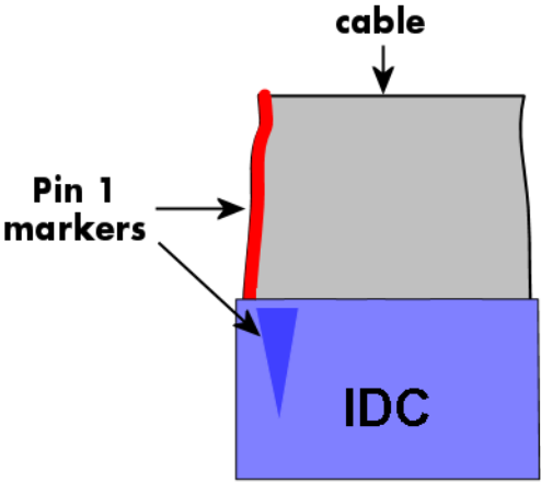
Image 98: IDC connector marking of pin 1
