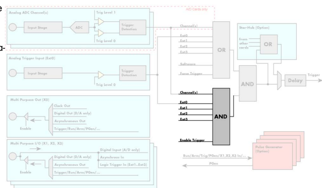
Image 62: Trigger overview - trigger AND mask
