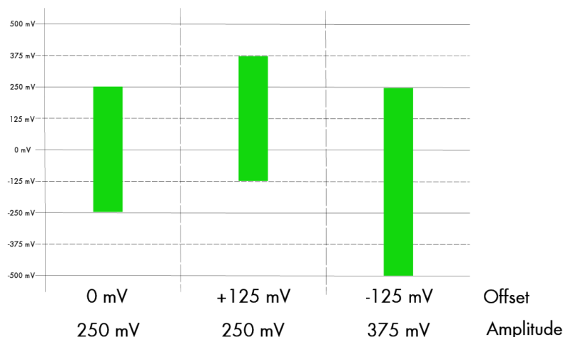
Image 45: output offset in relation to output signal and programmed amplitude
