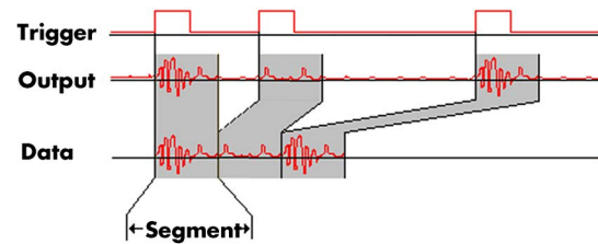
Image 69: Multiple Replay output and trigger timing diagram
