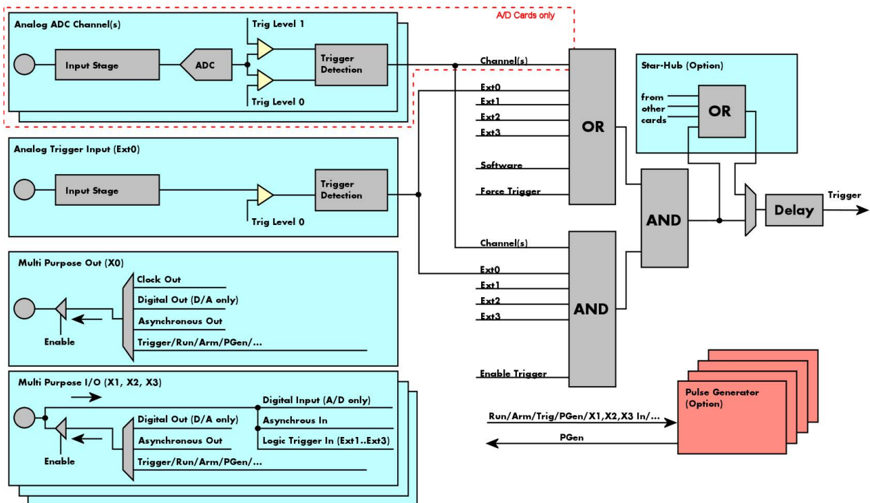
Image 59: M2p card trigger engine overview with the different trigger sources and trigger outputs
