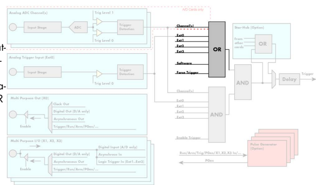
Image 60: Trigger overview - trigger OR mask
