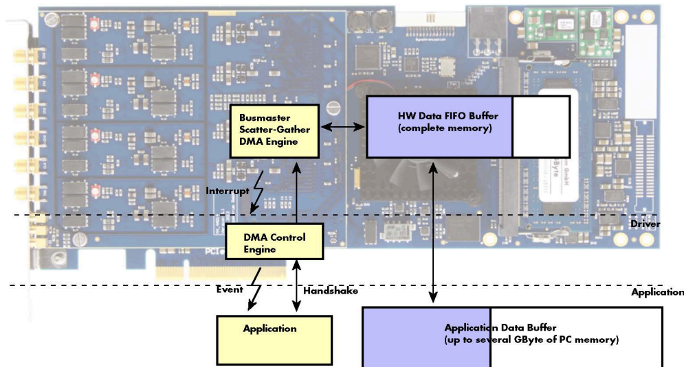
Image 56: Overview of buffer handling for DMA transfers showing and the interaction with the DMA engine
