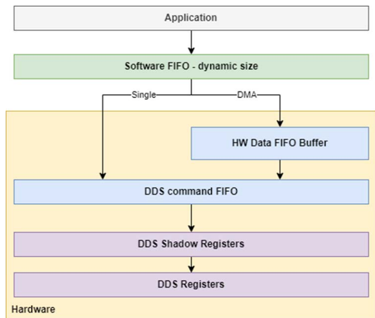
Image 80: The different FIFO buffers in DDS mode
