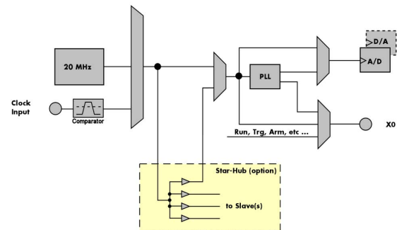
Image 58: Overview of M2p clock structure with optional star-hub
