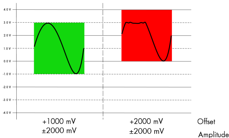
Image 46: output signal when exceeding maximum available output range
