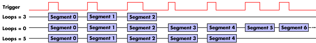
Image 72: timing diagram of Multiple Replay FIFO mode with different loops settings
