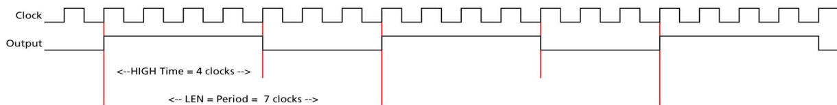
Image 87: timing diagram illustrating the basic pulse parameters
