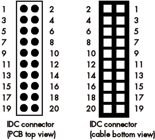
Image 97: IDC connector pinning of standard digital connection
