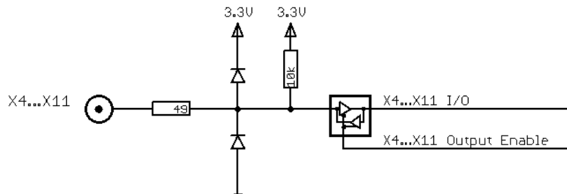
Image 102: electrical connection of additional I/O lines on connection DigBNC (digitizerNETBOX)
