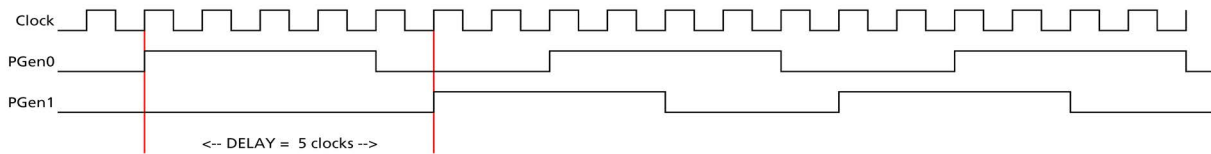
Image 88: timing diagram illustrating delaying a pulse generator output
