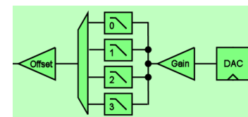
Image 47: output stage with selectable filters
