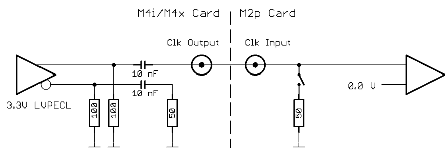
Image 103: Electrical interfacing of clock connections between M2p and M4i cards
