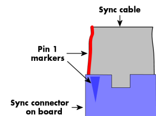
Image 10: Star-Hub connector pin-1 marker
