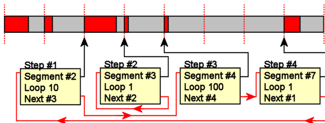
Image 78: sequence mode changing sequence on-the-fly
