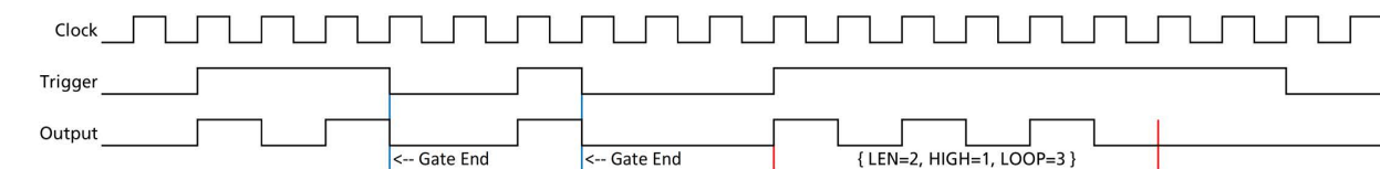
Image 91: timing diagram illustrating the pulse generator gated output mode
