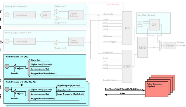
Image 67: overview block diagram of multi-purpose I/O lines
