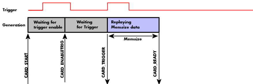
Image 52: timing diagram of single replay mode with commands and status changes
