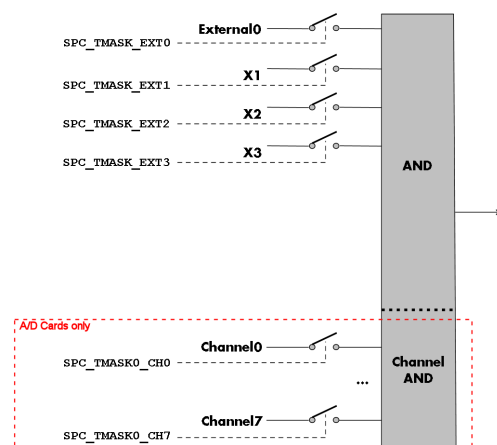
Image 63: trigger AND mask details
