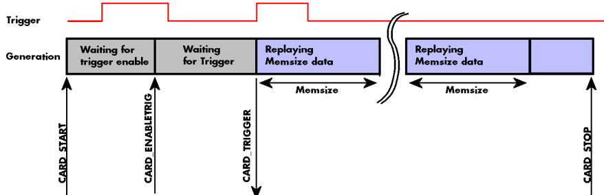
Image 54: timing diagram of continuous replay mode stopped by user with commands and status changes
