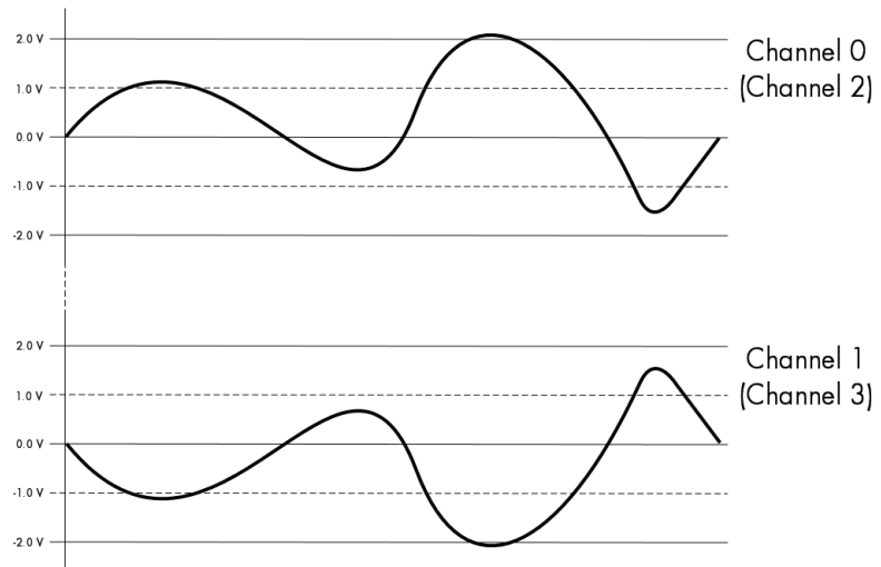
Image 48: schematic of differential output mode
