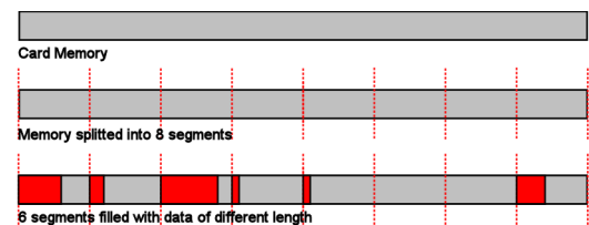
Image 76: Sequence Mode: Segment definition in card memory
