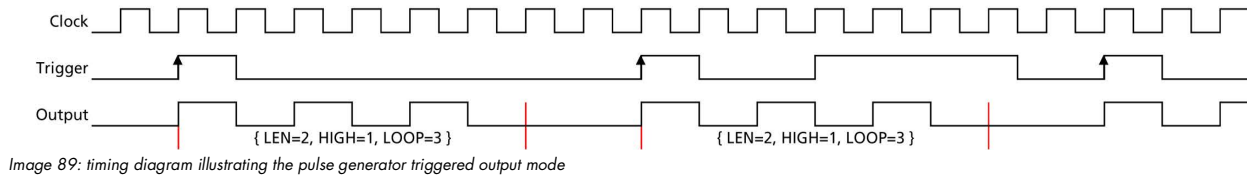
Image 89: timing diagram illustrating the pulse generator triggered output mode
