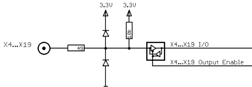
Image 101: electrical connection of additional I/O lines on connection DigSMB
