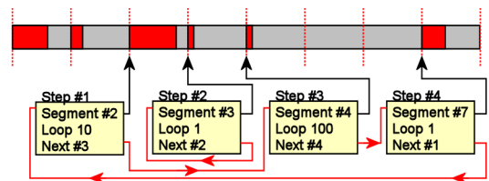
Image 77: Sequence mode: steps and step looping
