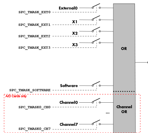
Image 61: trigger OR mask details
