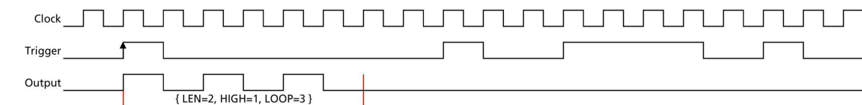
Image 90: timing diagram illustrating the pulse generator single-shot triggered output mode
