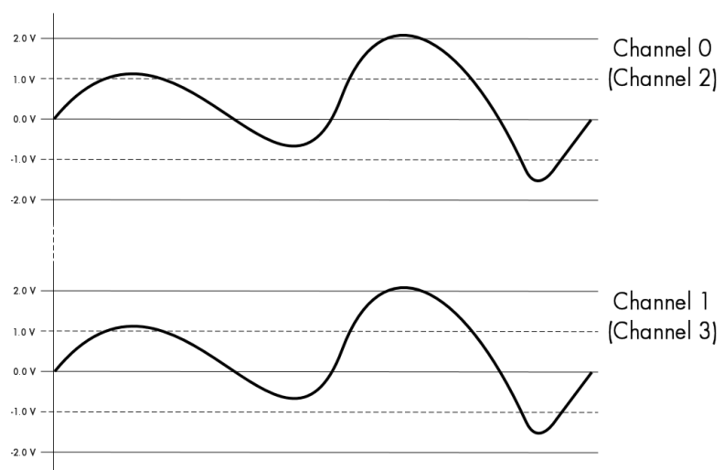
Image 49: schematics of double output mode
