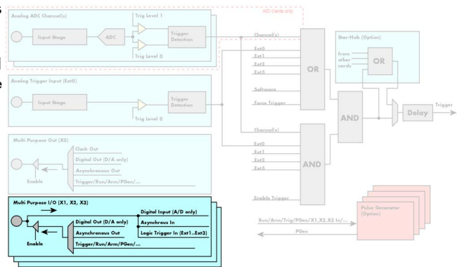
Image 66: trigger engine overview and multi purpose trigger
