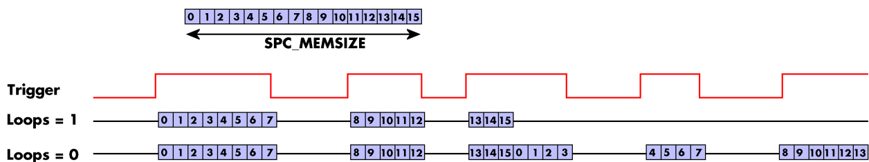
Image 74: timing diagram of Gated Replay mode depending on different loops settings
