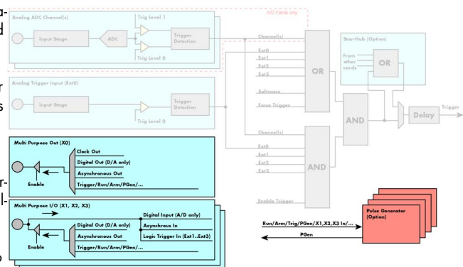
Image 85: overview block diagram of multi-purpose I/O lines and pulse generators
