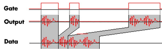
Image 73: Gated Replay timing diagram in relation to gate signal
