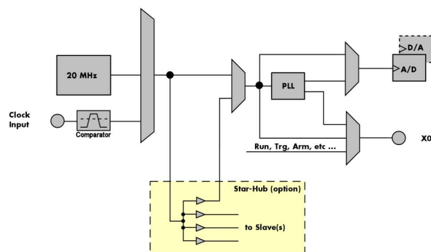
Image 92: Drawing of star-hub clock engine location and interaction with card clock
