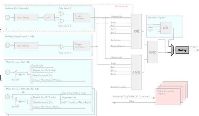
Image 64: M2p trigger engine overview and delay trigger
