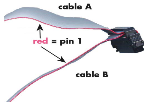
Image 96: location of pin 1 on the standard 40-pole flat ribbon cable
