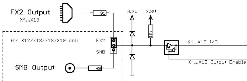
Image 100: electrical connection of additional I/O lines on connection DigFX2
