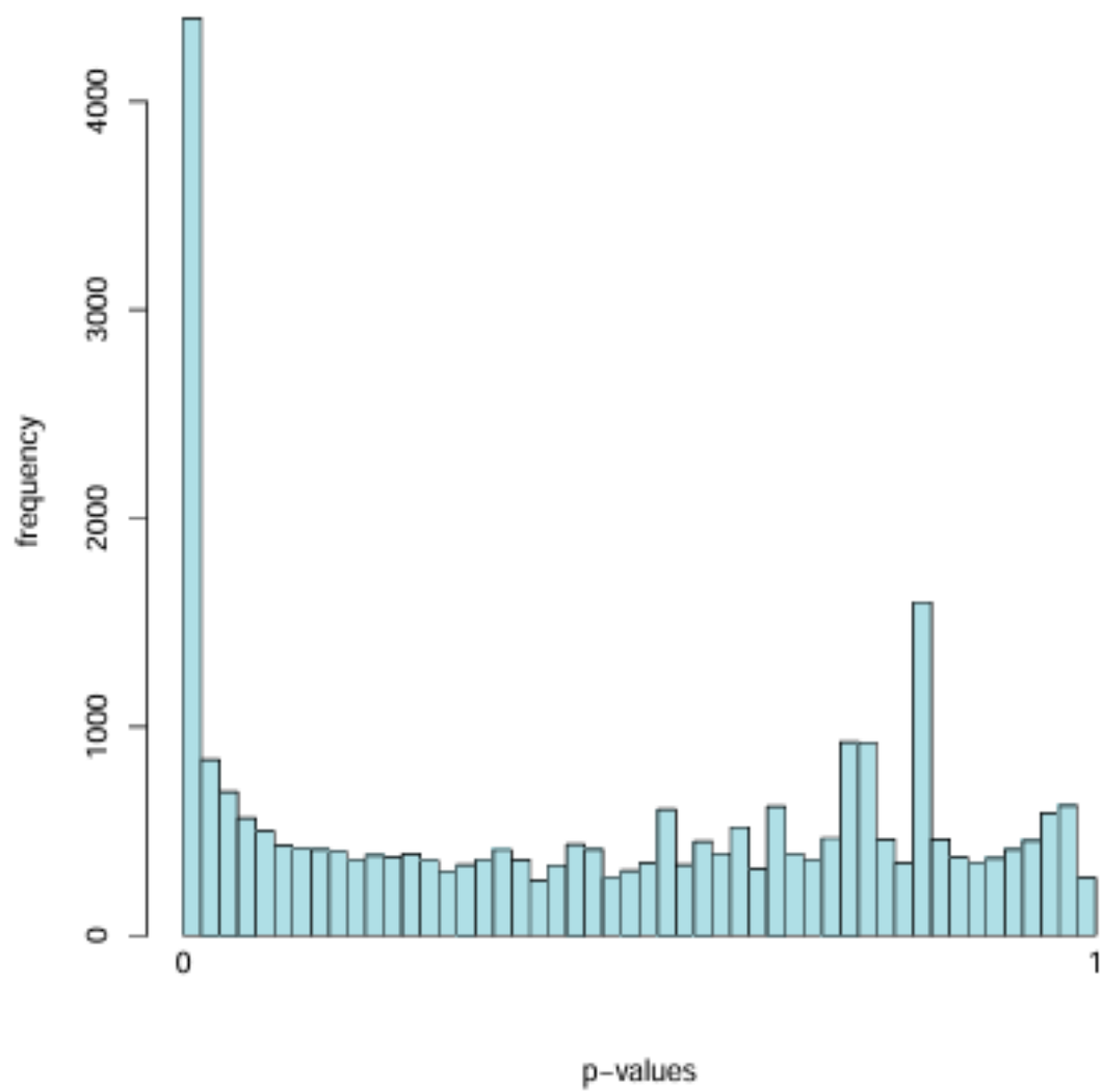
Histogram of p-values for Condition: Control vs Infected
