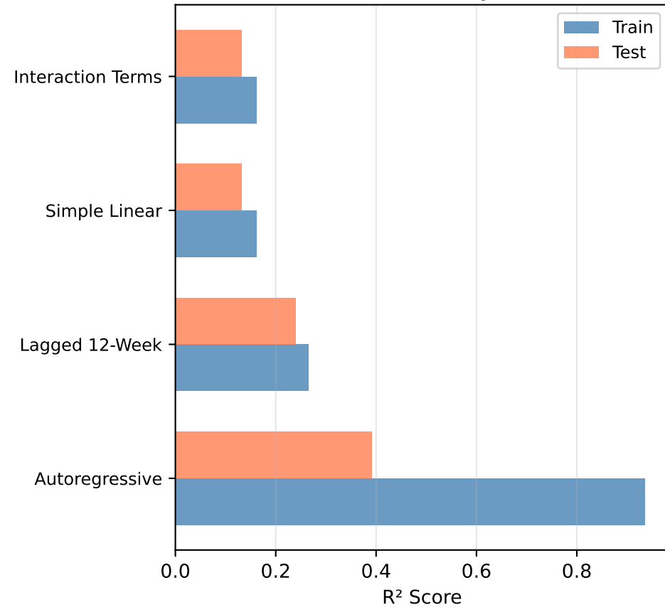
Model R 2 Comparison
