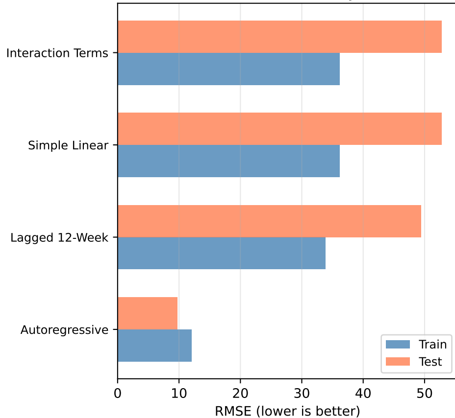
Model RMSE Comparison
