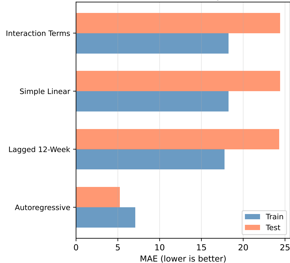
Model MAE Comparison
