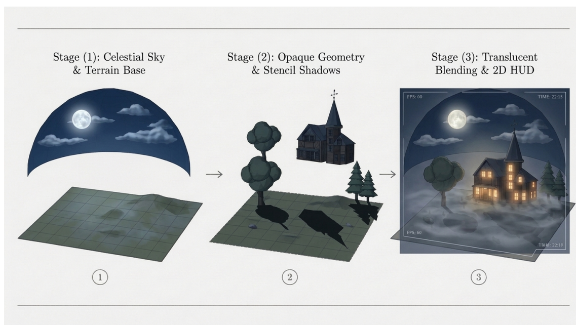
Figure 22: Multi-pass render composition sequence: celestial sky and moon, terrain and architecture geometry, stencil shadow projections, translucent alpha blending, and orthographic UI overlay.
