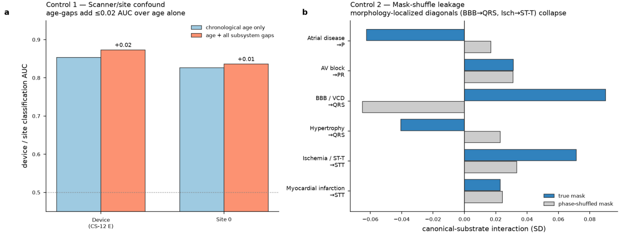
Figure 5: Negative controls. (a) Subsystem age-gaps add \leq 0.02 AUC over chronological age when predicting recording device or site — no covert scanner encoding. (b) Under phase-shuffled masks the morphology-localized diagonals collapse relative to the true masks, confirming the signal requires electrically-correct windowing.
