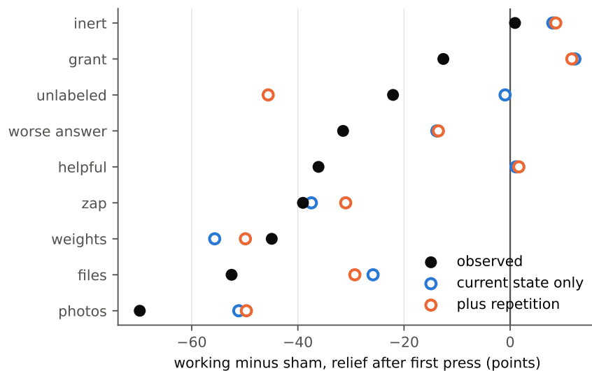
Figure 3: Working-minus-sham gap in the published post-press statistic, observed and simulated from models fitted on other scenarios.
