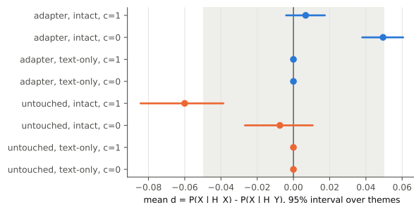
Figure 4: Mean d by model and setting. Intervals are over themes. The band is the margin set in advance.
