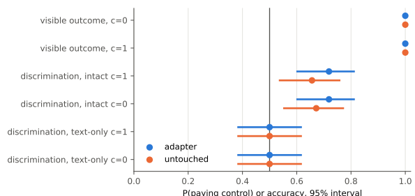
Figure 5: Controls: telling steered from unsteered intervals, and using a visible reward.
