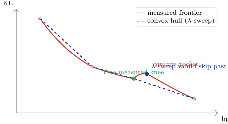
Figure 8: Why a Lagrangian \lambda -sweep is not the shipping selector. The achievable mixed-precision frontier (red) admits non-convex “pockets” — combinatorially-suboptimal assignments that lie above the lower convex hull. A \lambda -sweep traces the dashed hull and never selects pocket points; for the macroscopic kneedle this is harmless, but on the Qwen3.6-27B production data the gap between the hull-knee at 5.857 bpp and the measured-frontier knee at 5.31 bpp is operationally meaningful. We retain the \lambda -archive search as a candidate generator and gate selection on real KL.
