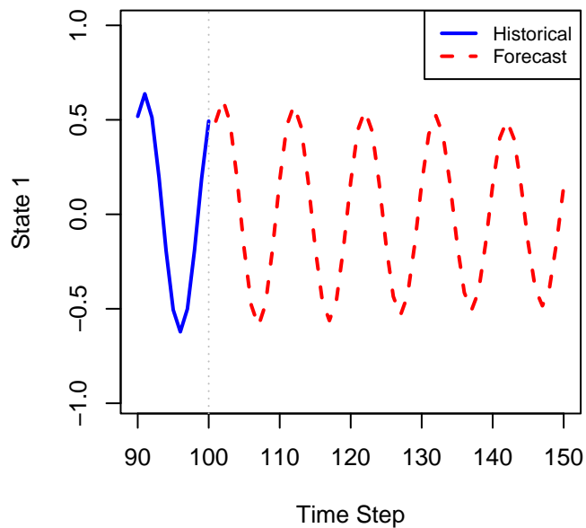
x_0 = \text{Mid-point} : Interpolation Test
