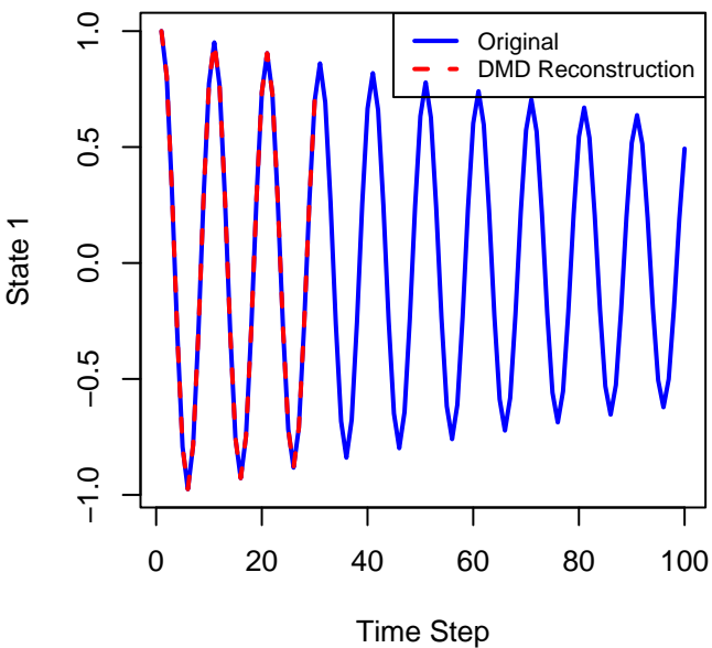
x_0 = \text{Custom State } [0.5, 0.3]
