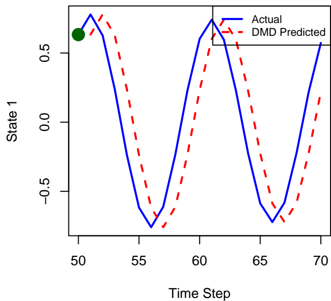
x_0 = \text{Mid-point} : Interpolation Test
