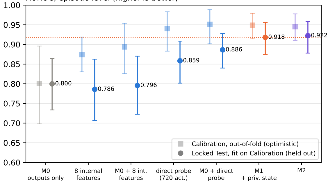
AUROC, episode level (higher is better)
