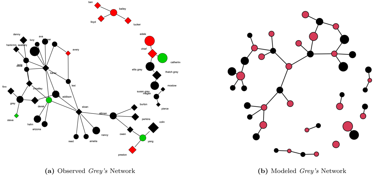
Figure 1: Two visualizations of Grey's Anatomy hookup network data from ergm tutorial. Panel A represents the "observed" data with identities and multiple attributes attached (size=age, color=race, shape=gender). Panel B represents network generated from the modeled results, including only those features that are part of the model (node color=gender). This example is adapted from (Lind 2012).
