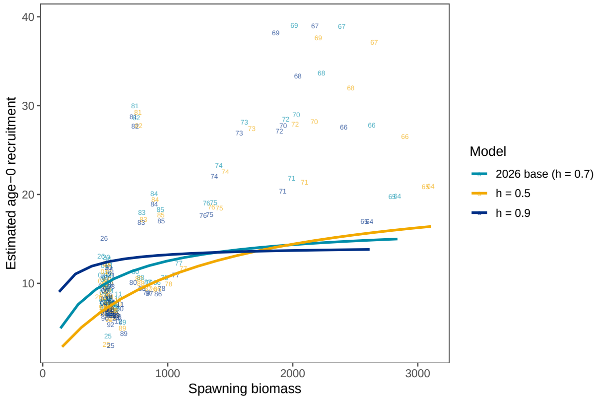
Figure 7: Fitted stock–recruit curves and annual estimates for the 2026 base model and two fixed-steepness sensitivities, overlaid in one panel and coloured by model. Estimates are identified by two-digit year labels.
