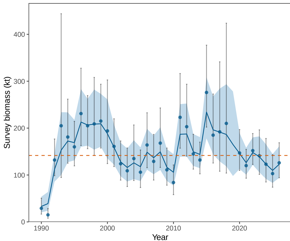
Figure 2: REMA-smoothed survey biomass estimates for M. paradoxus through 2026. The dashed line is the geometric mean of predicted biomass over 1990–2026.
