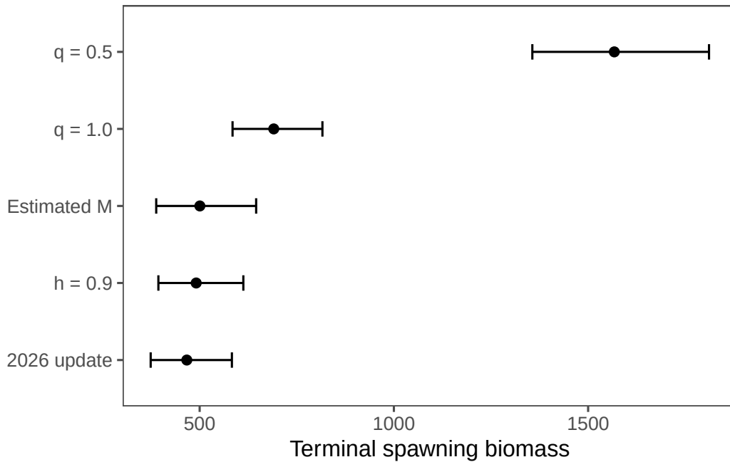
Figure 5: Terminal spawning biomass for the converged 2026 models.
