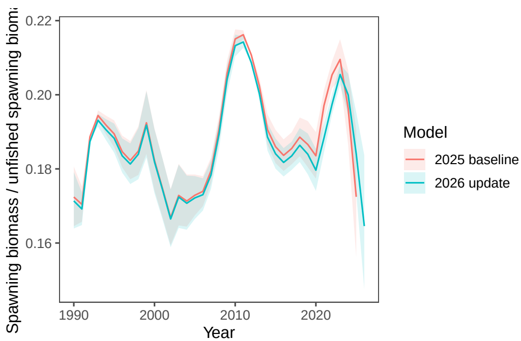
Figure 4: Estimated depletion from the 2025 baseline and 2026 update.
