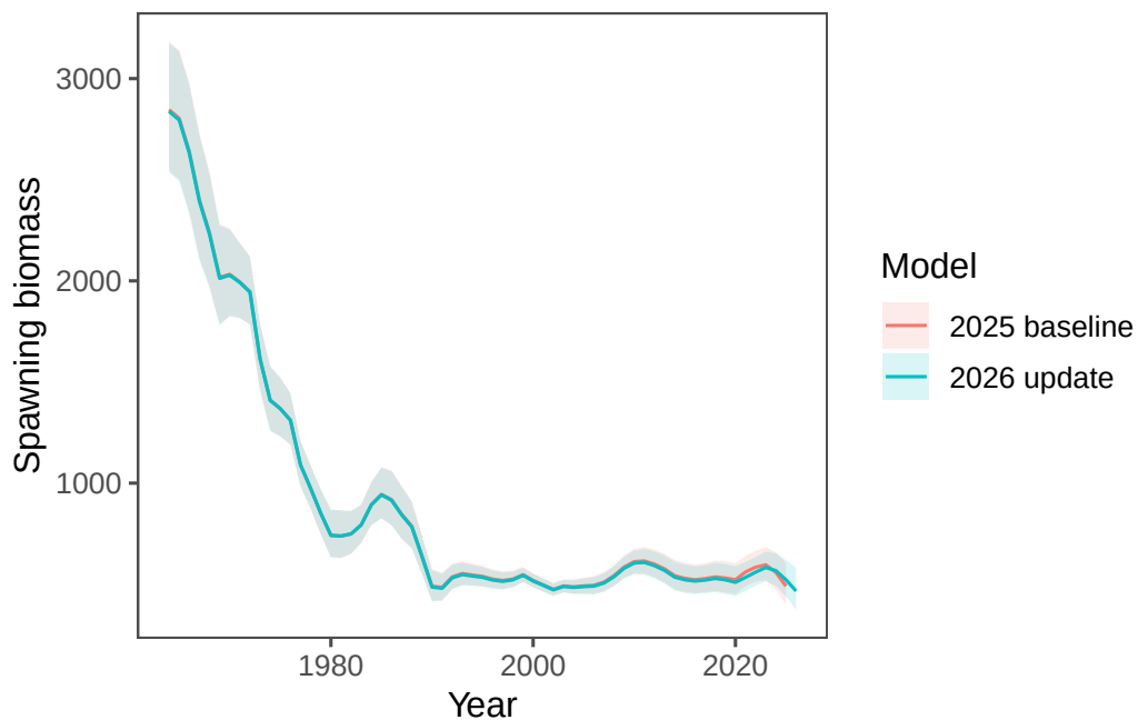
Figure 3: Spawning biomass from the unchanged 2025 model and the 2026 data update.
