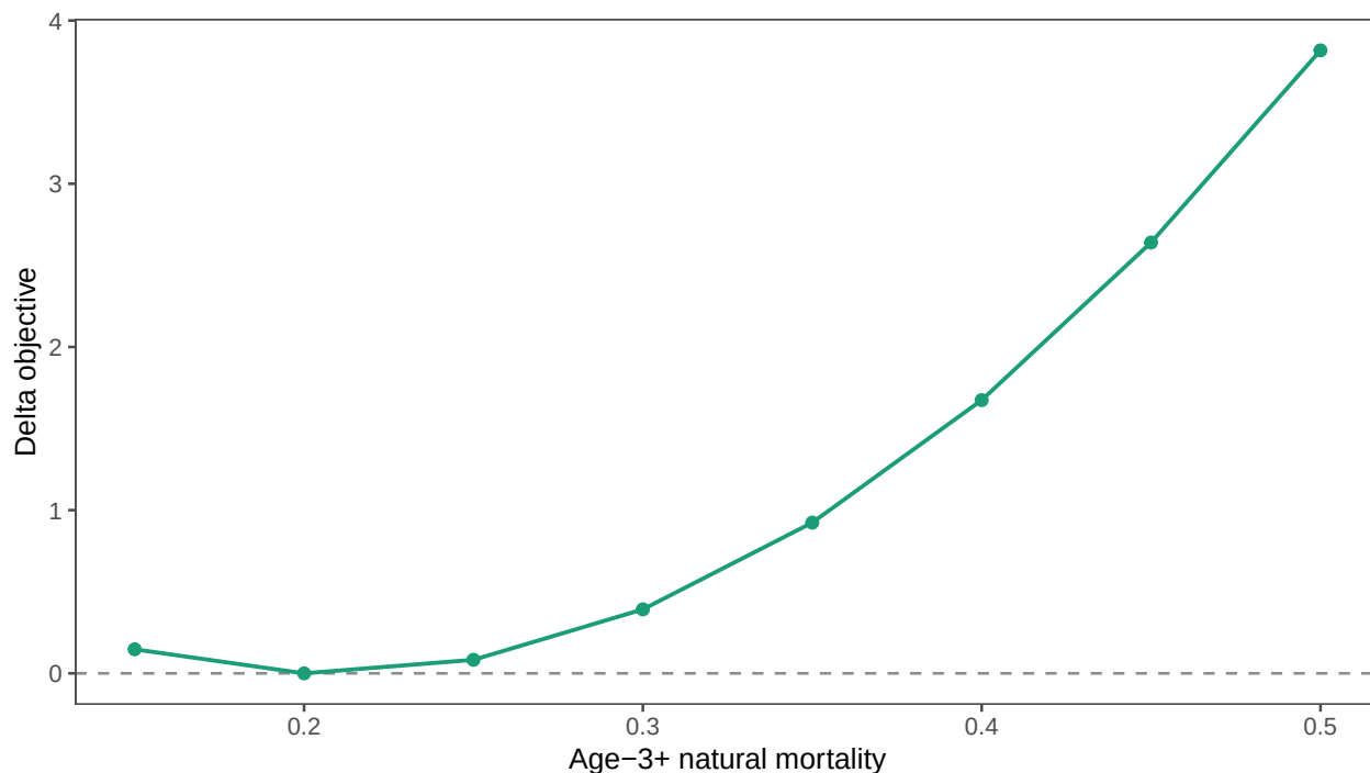
Figure 23: Profile of age-3-and-older natural mortality for the Rceattle 5.8.1 configuration. Points are evaluated grid values and the vertical axis is objective difference from the grid minimum.
