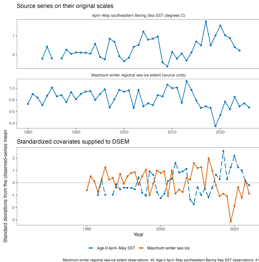
Figure 14: Physical-forcing source series and the standardized, cohort-aligned values supplied to the Rceattle-DSEM suite.
