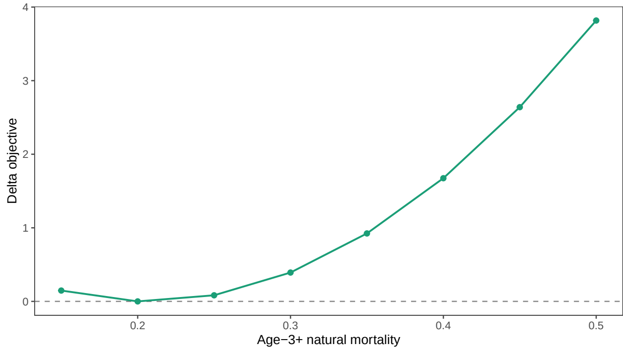
Figure 12: Profile of age-3-and-older natural mortality for the Rceattle 5.8.1 configuration. Points are evaluated grid values and the vertical axis is objective difference from the grid minimum.
