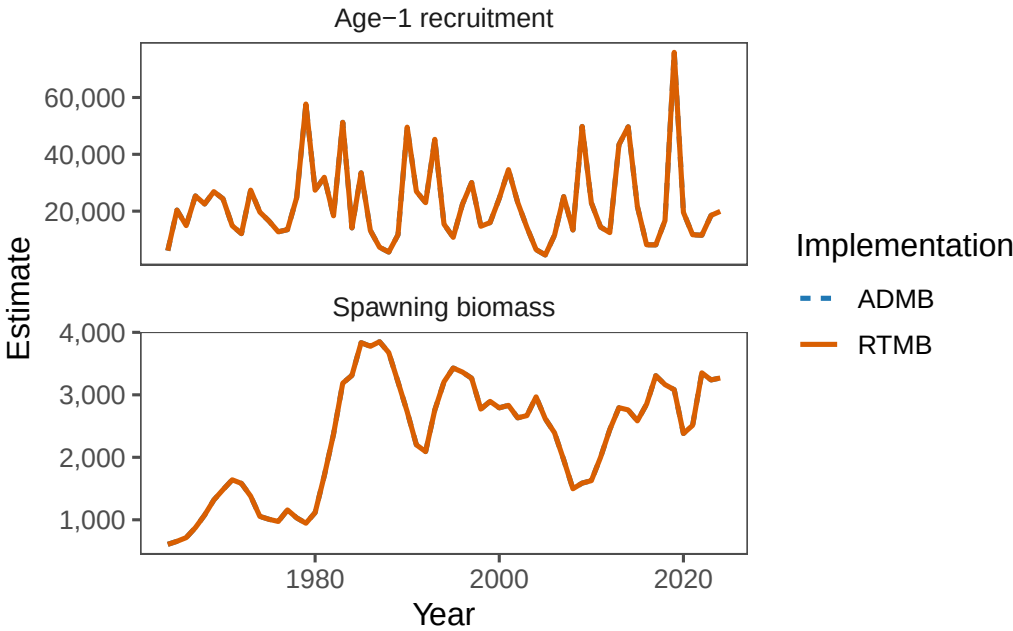
Figure 4.1: Spawning biomass and age-1 recruitment from RTMB and ADMB at the same ADMB maximum-likelihood parameter estimates. The two implementations are visually indistinguishable at the plotted scale. Select the figure to open it in the lightbox.
