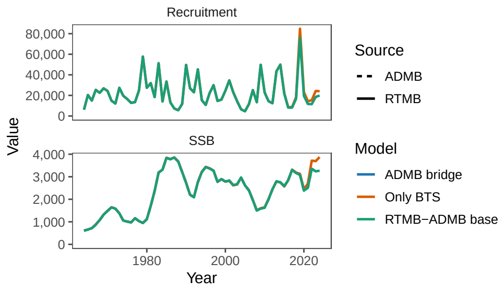
Figure 7.2: Shared RTMB and ADMB bridge time series for spawning biomass and recruitment, including the Only BTS RTMB sensitivity model with ATS and AVO survey index likelihoods excluded.
