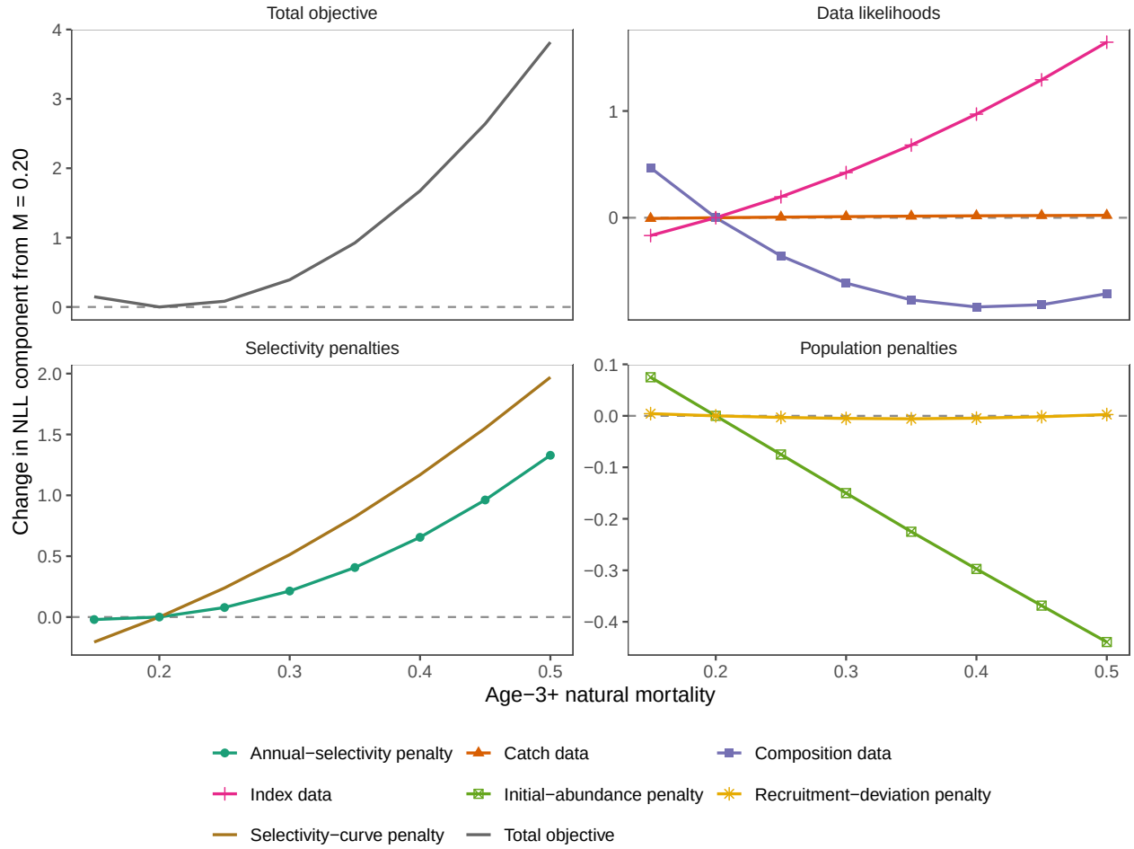
Figure 12: Component decomposition of the age-3-and-older natural-mortality profile. Each curve is the change in that NLL component relative to its value at M = 0.20 . Positive values favor M = 0.20 over the plotted value; negative values favor the plotted value. Components in the three lower panels sum to the total objective change in the upper-left panel.
