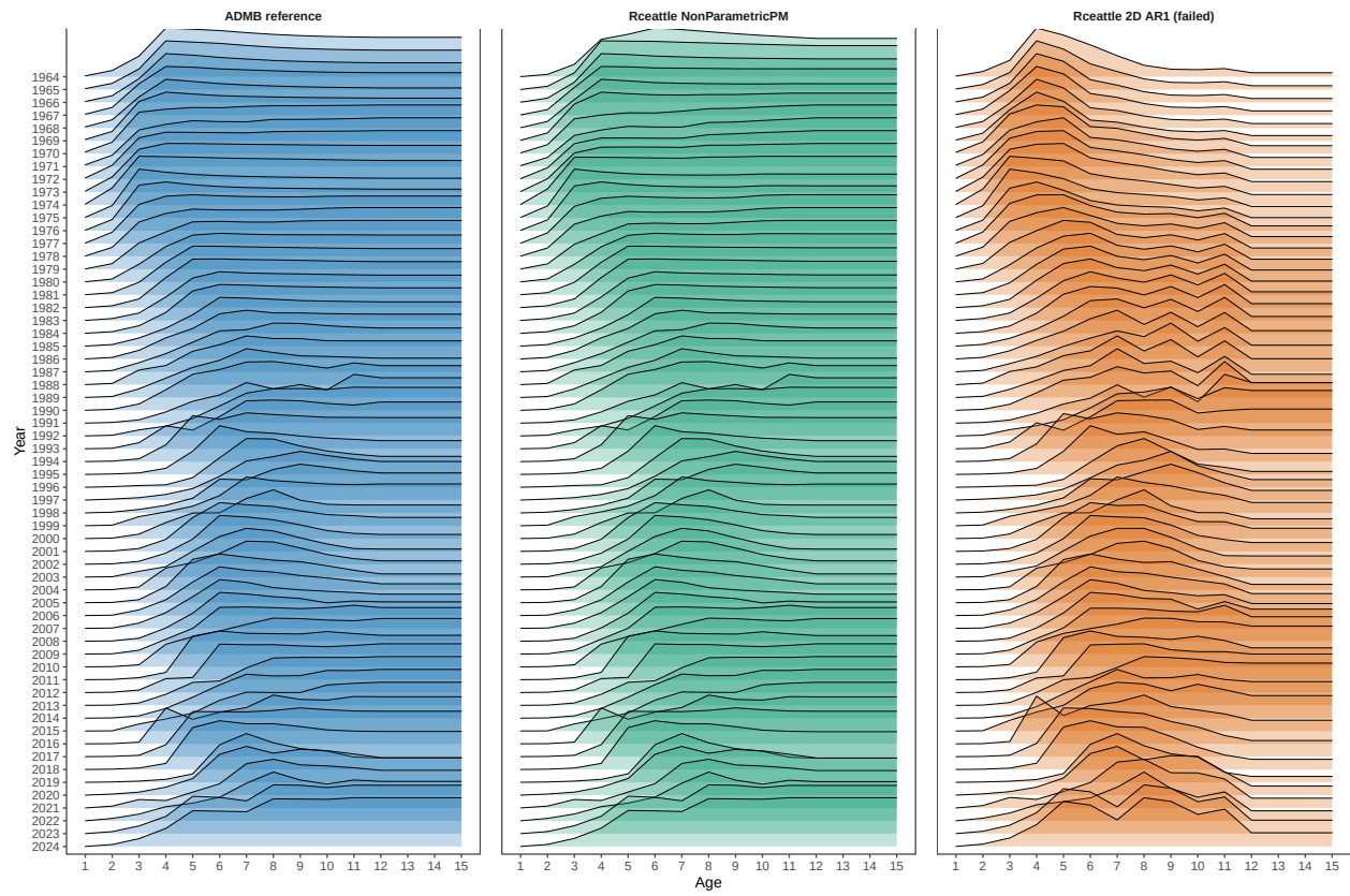
Figure 13: Development comparison of relative fishery selectivity for ADMB, the Rceattle configuration, and the failed 2D age-by-year AR1 sensitivity.
