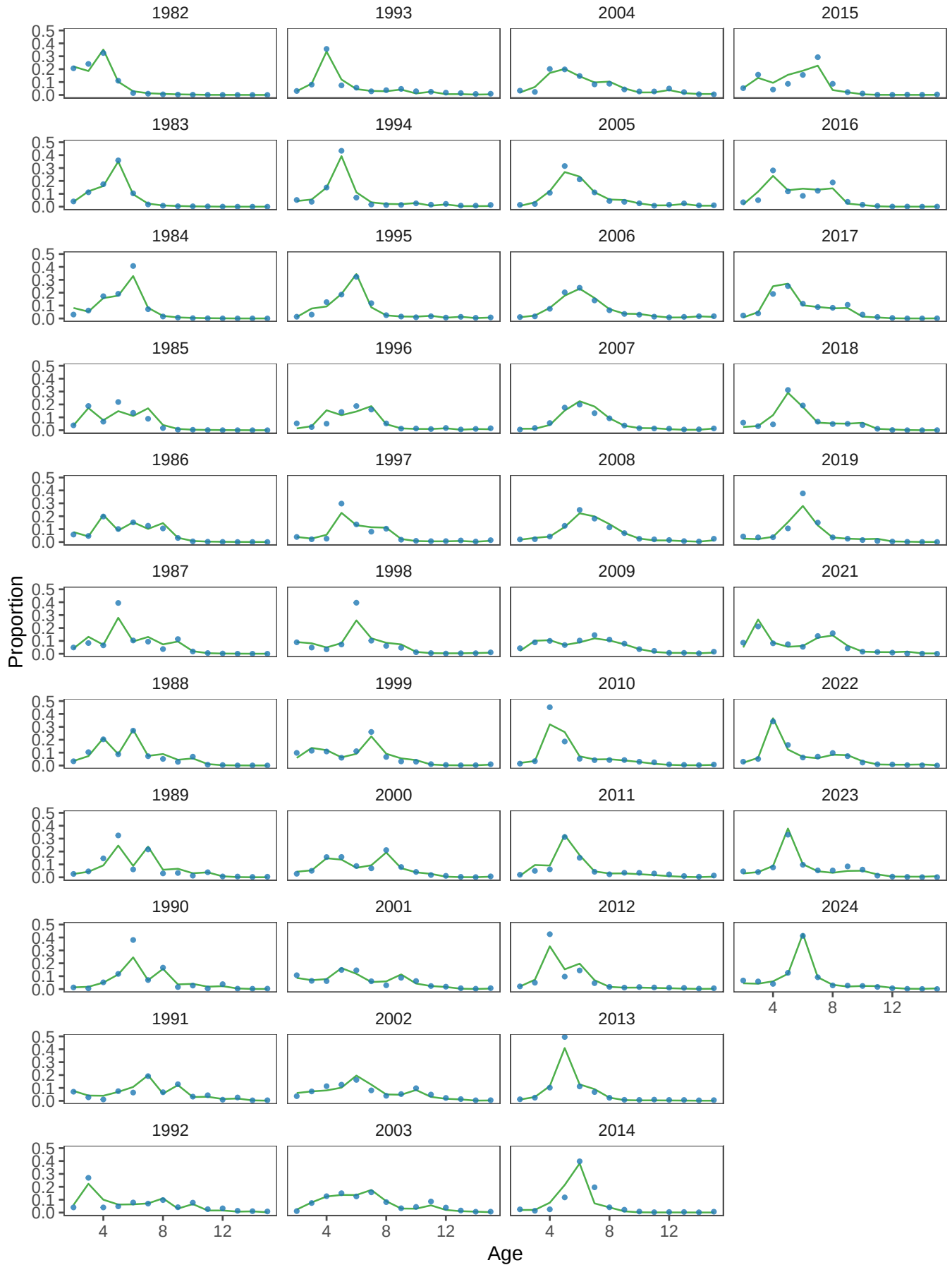
Figure 5.6: Observed and expected BTS age-composition patterns from the saved RTMB-ADMB model, faceted by year.
