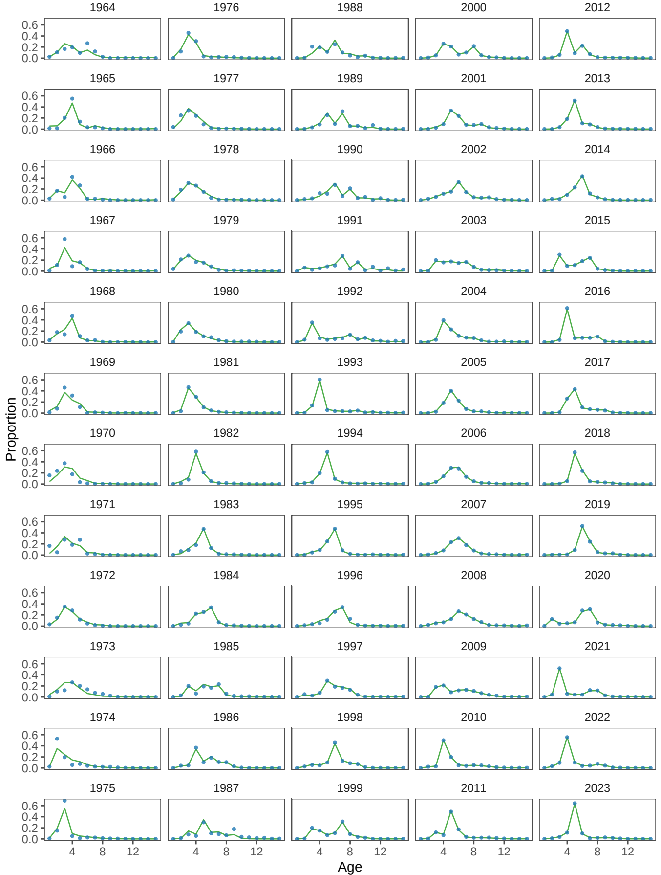
Figure 5.5: Observed and expected fishery age-composition patterns from the saved RTMB-ADMB model, faceted by year.
