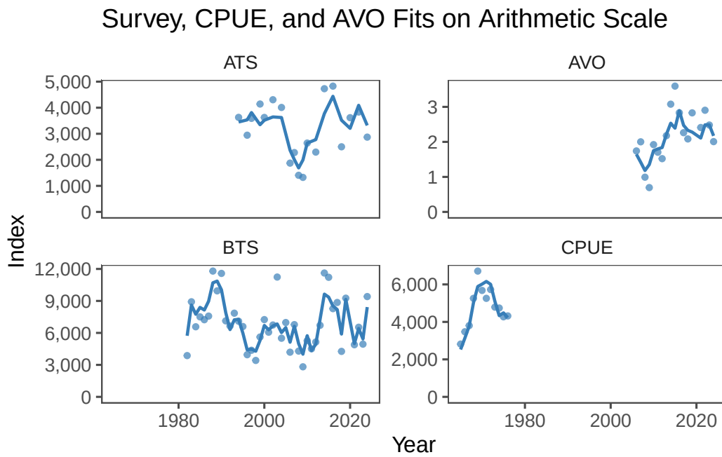
Figure 5.3: Observed and predicted index series from the saved RTMB-ADMB model, shown on arithmetic scales with separate facet axes.
