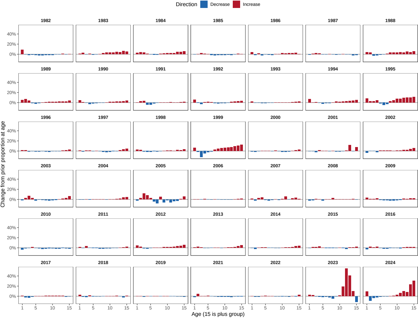
Figure 10.1: Percent change in BTS proportions at age from the original BTSPProp.csv series to the revised tinyVAST_props_new.csv series for each matched historical survey year. Positive bars indicate a larger tinyVAST proportion and negative bars indicate a smaller tinyVAST proportion. Age 15 is the plus group; no BTS survey occurred in 2020.
