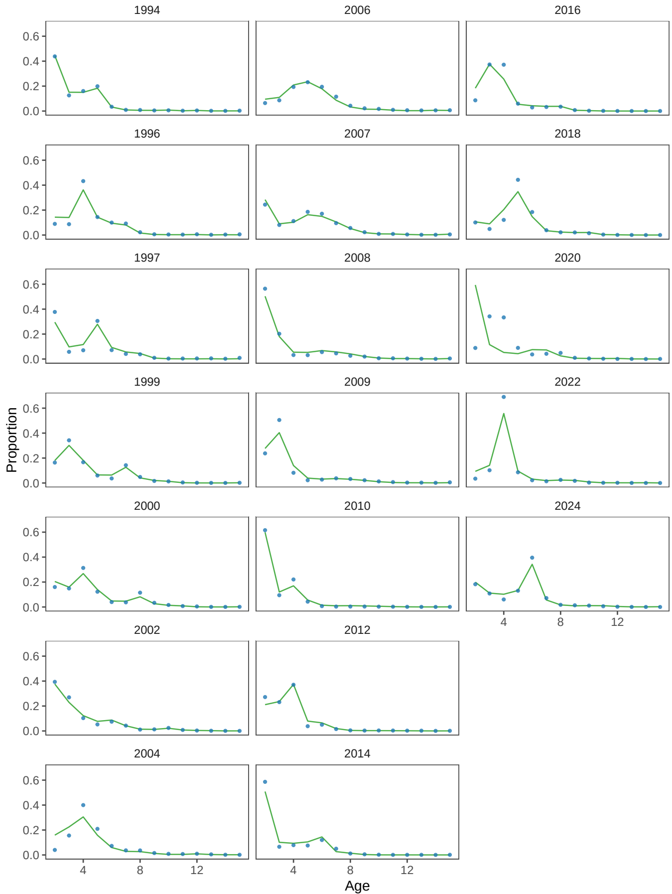
Figure 5.7: Observed and expected ATS age-composition patterns from the saved RTMB-ADMB model, faceted by year.
