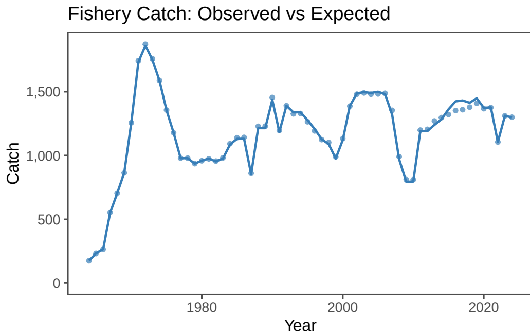
Figure 5.2: Observed fishery catch and predicted catch from the saved RTMB-ADMB model.
