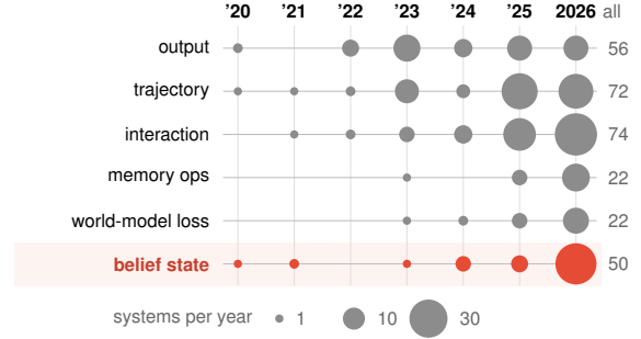
Fig. 6 | Where credit has gone, 2020–2026. Bubble area counts systems crediting each object per year; the right column gives totals (Table 16). In another 221 no object receives a signal. Credit reached the belief state mostly in 2026, and only ReBel and ABBEL take its test from the agent’s own observations.
