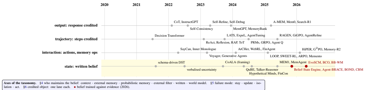
Figure 7: Where credit has gone, 2020–2026. Lanes are credited objects; Table 13 lists every screened system. Written beliefs exist from dialogue state tracking onward, but until 2026 they are credited by task outcome or not trained at all; the red points are the first to give the belief its own learning signal.
