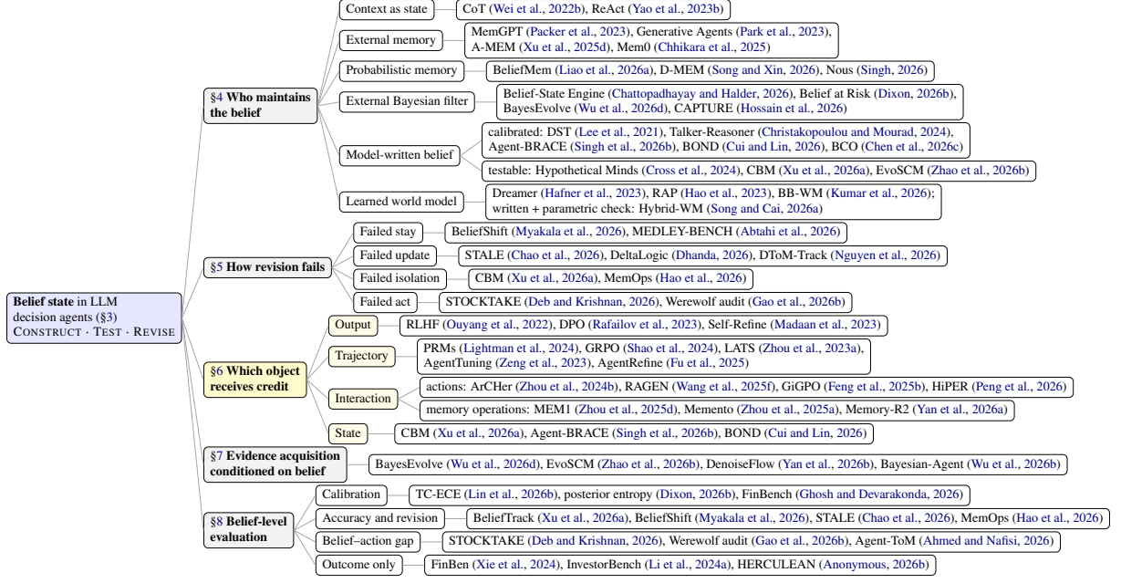
Figure 1: Taxonomy of the survey with representative systems by year. The credited object (yellow) is the axis every method is placed on; Table 13 in the appendix places every screened system.
