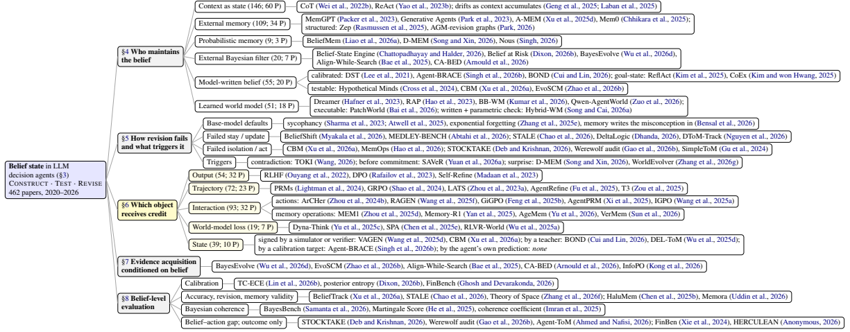
Figure 1: Taxonomy of the survey with representative systems. Counts in parentheses are the included papers coded in each class and, after the semicolon, how many of them are peer-reviewed (Appendix A); the three operations are the axes, and the credited object (yellow) is where the gap the survey identifies lies: its last leaf is empty. Table 15 in the appendix places every included paper.
