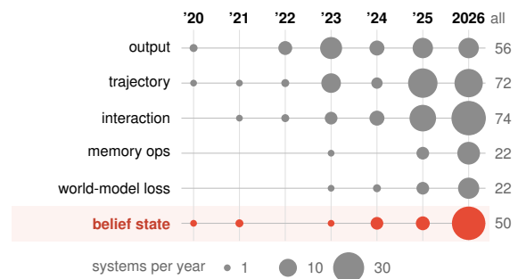
Fig. 6 | Where credit has gone, 2020–2026. Bubble area counts systems crediting each object per year; the right column gives totals (Table 15). Another 221 train nothing. Credit reached the belief state mostly in 2026, and only ReBel and ABBEL take its test from the agent’s own observations.
