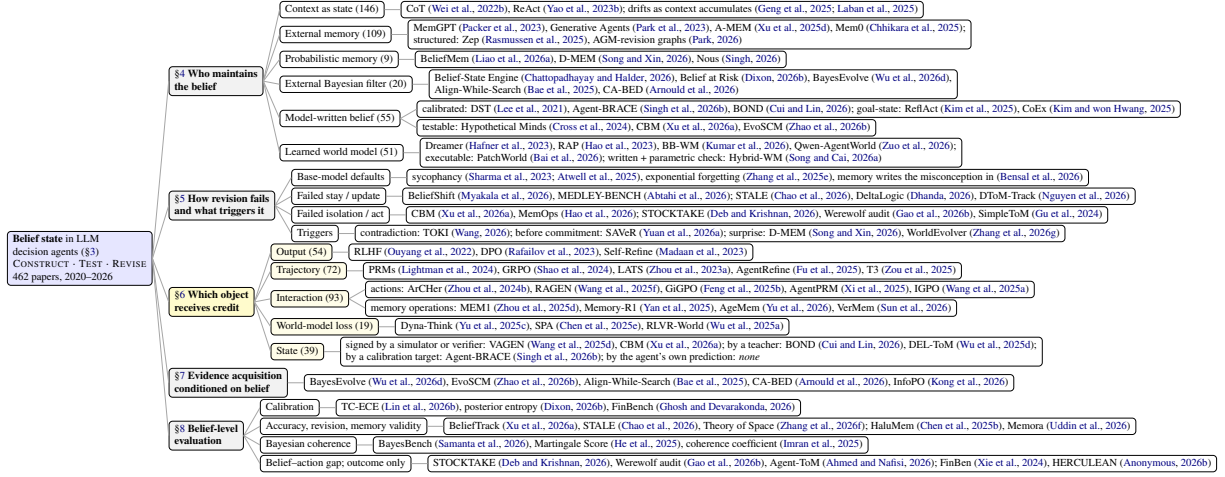
Figure 1: Taxonomy of the survey with representative systems. Counts in parentheses are the number of included papers coded in each class (Appendix A); the credited object (yellow) is the axis every method is placed on, and its last leaf is empty. Table 15 in the appendix places every included paper.
