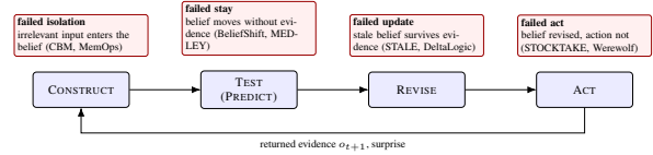
Figure 3: Where the four failure modes of Section 5 occur on the construct–test–revise–act cycle. Only a testable belief lets returned evidence be routed to the operation that failed rather than to the action.
