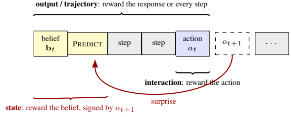
Figure 4: The credited object on one span of a trajectory: output and trajectory credit reach generated text, interaction credit reaches the action, state credit reaches the written belief with a sign from the observation returned after the action.
