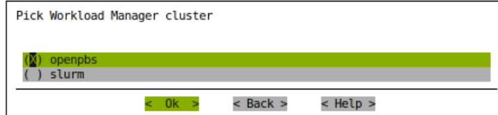
Figure 8.6: Auto Scaler Setup Workload Manager Selection
