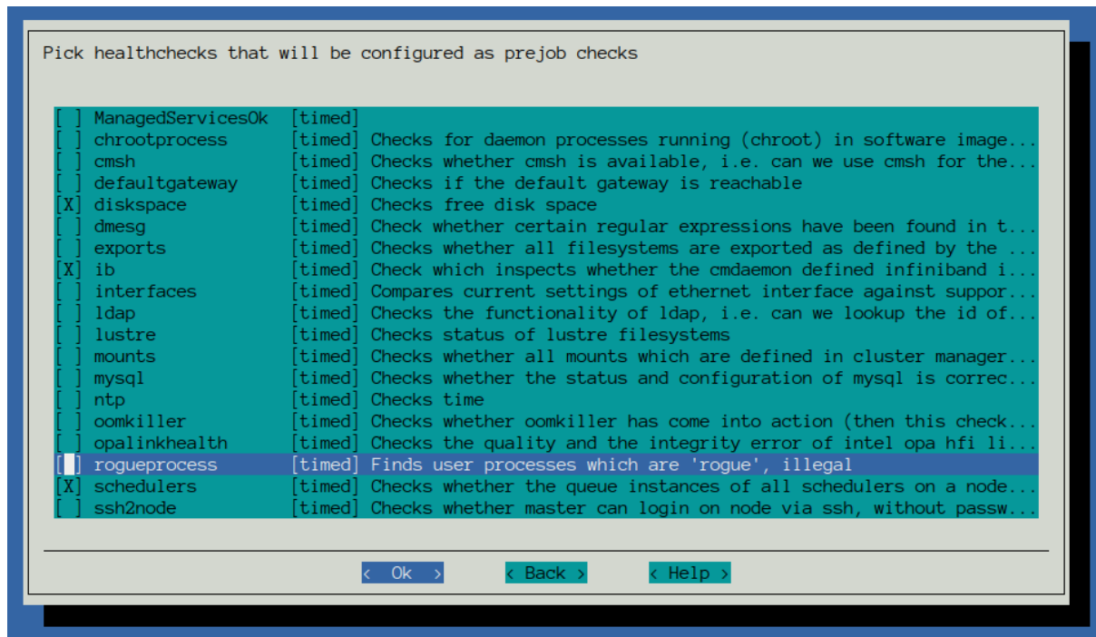
Figure 7.37: Prejob healthcheck selection in the cm-wlm-setup screen
