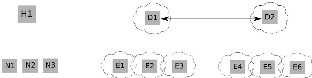
Figure 10.34: Backup Flow For Offloaded Monitoring With HA Edge Director Nodes
