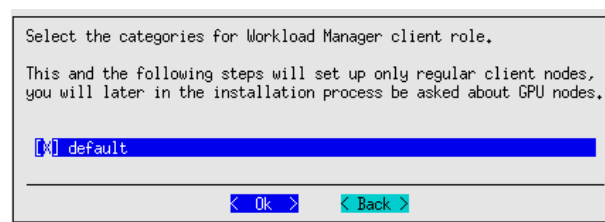
Figure 7.4: Slurm with cm-wlm-setup : WLM Client role category configuration screen
