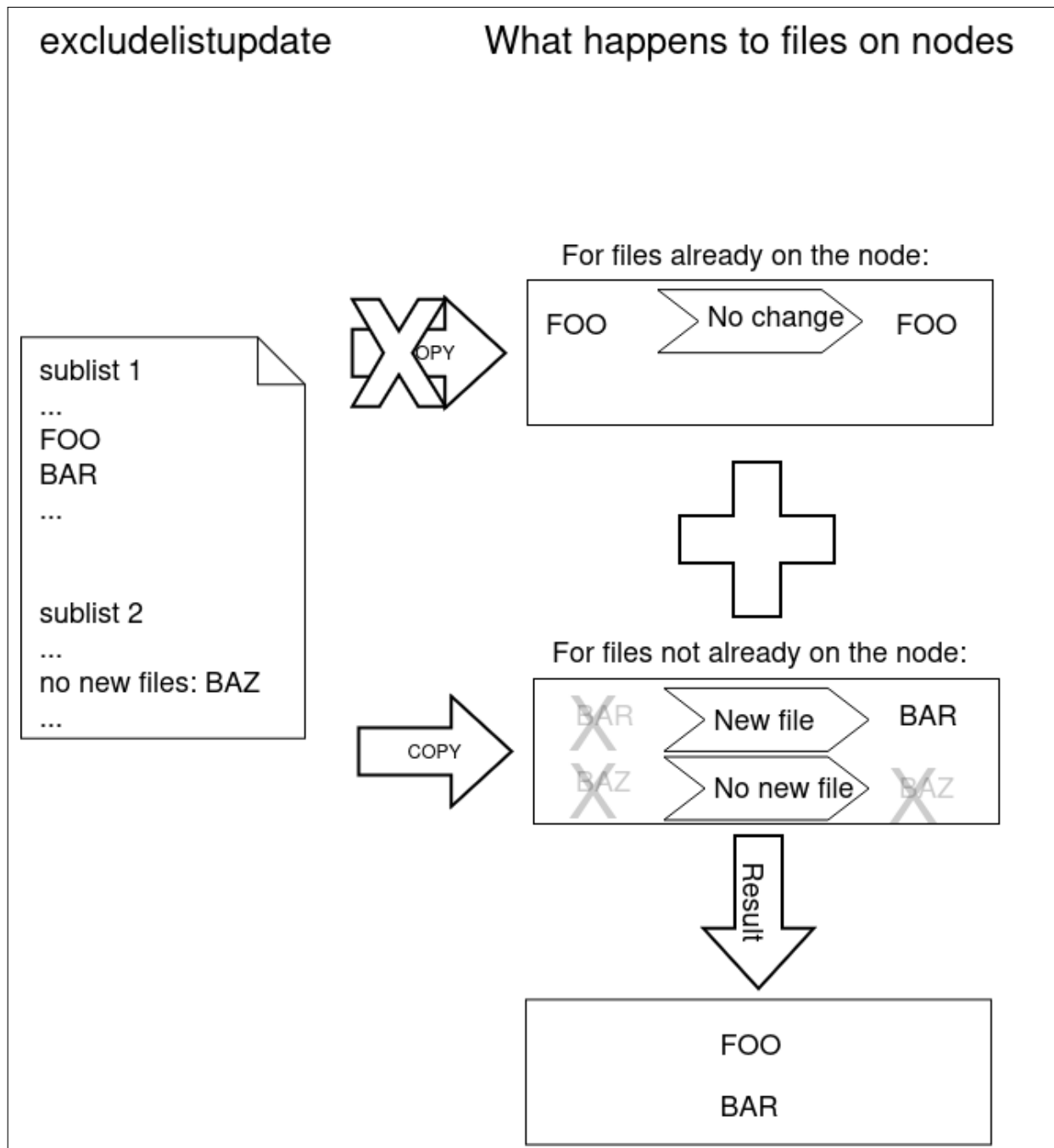
Figure 5.18: Exclude list logic
