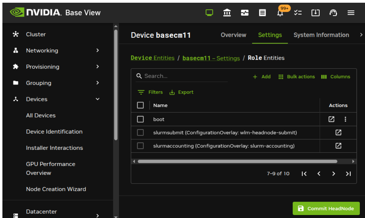
Figure 7.20: Roles seen on head node in Base View
