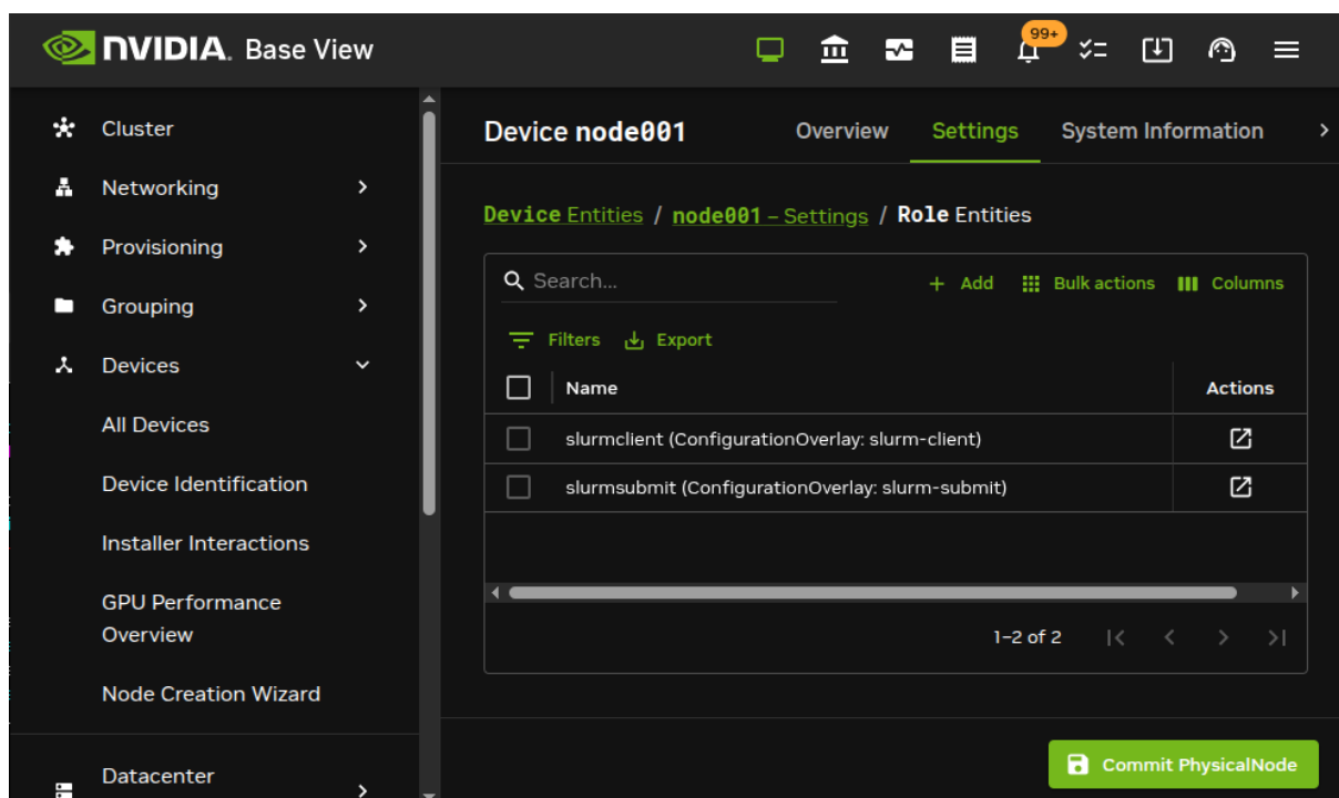
Figure 7.21: Roles seen on regular node in Base View
