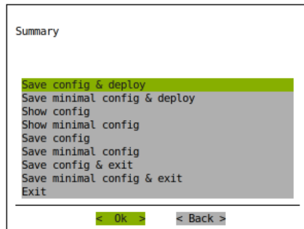
Figure 7.13: cm-wlm-setup TUI summary screen
