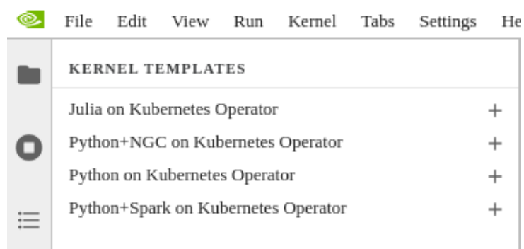
Figure 16.11: Jupyter Kernel Operator templates
