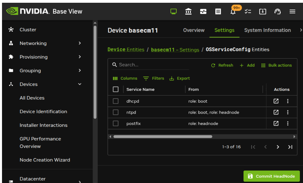
Figure 7.18: Services seen on head node in Base View
