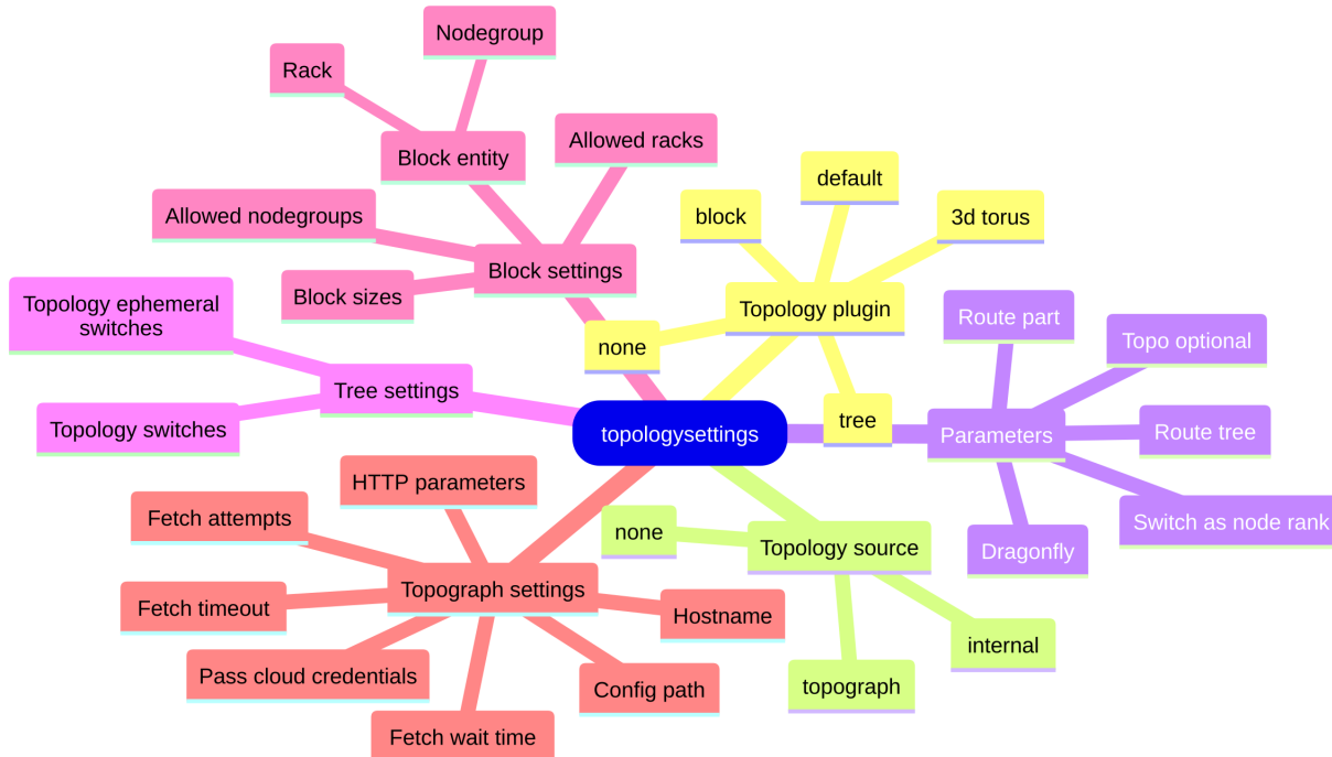
Figure 7.23: Visualization of settings under topologysettings
