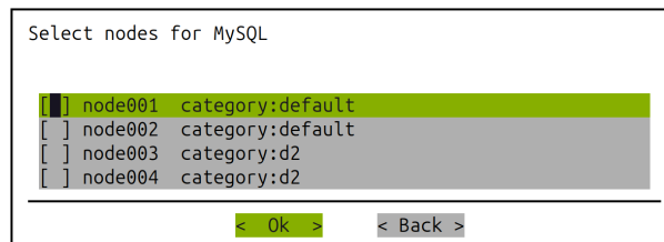
Figure 14.9: Base View MySQL Installation: Select nodes
