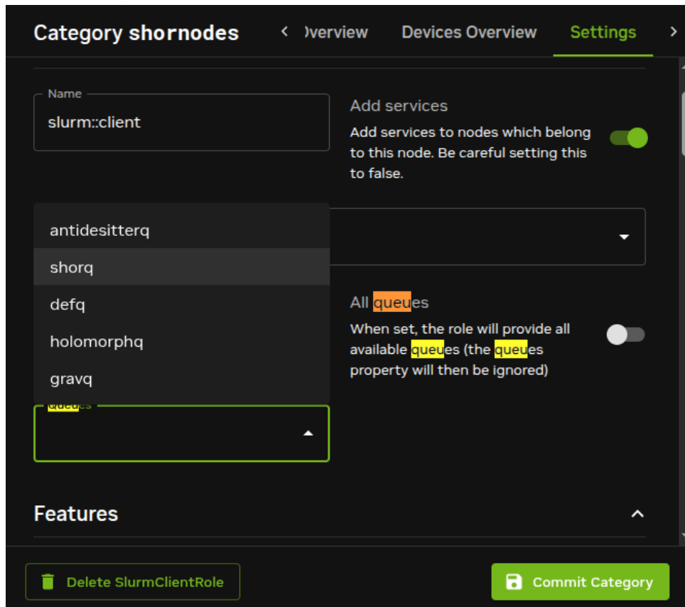
Figure 7.36: Setting a queue for a new category using Base View
