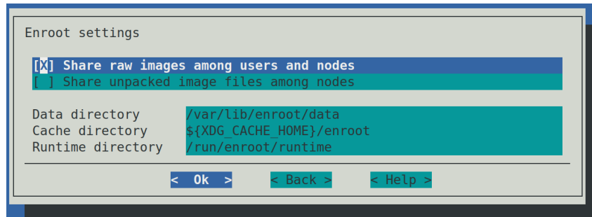
Figure 7.15: cm-wlm-setup Enroot settings screen
