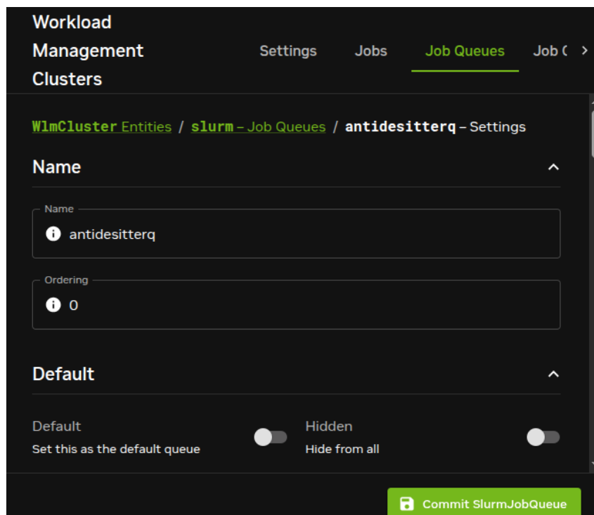
Figure 7.34: Workload manager queue parameters configuration
