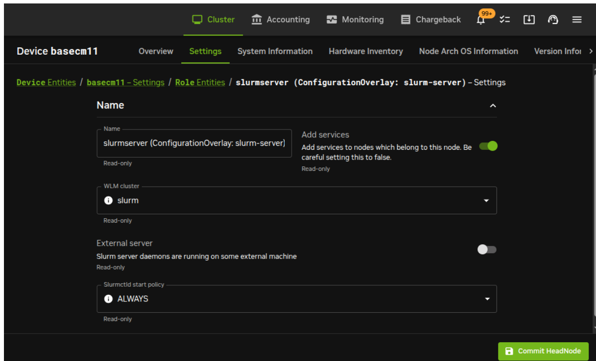
Figure 7.16: Workload management role assignment on a head node
