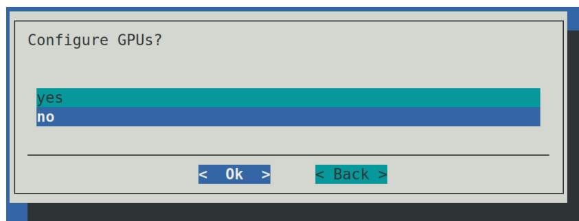
Figure 7.27: The screen prompting for GPU configuration in cm-wlm-setup
