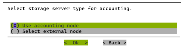
Figure 7.11: cm-wlm-setup selection of the type of node on which the Slurm accounting database runs
