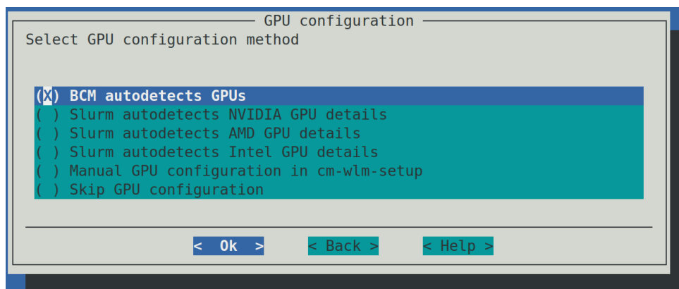
Figure 7.28: The GPU configuration screen of cm-wlm-setup
