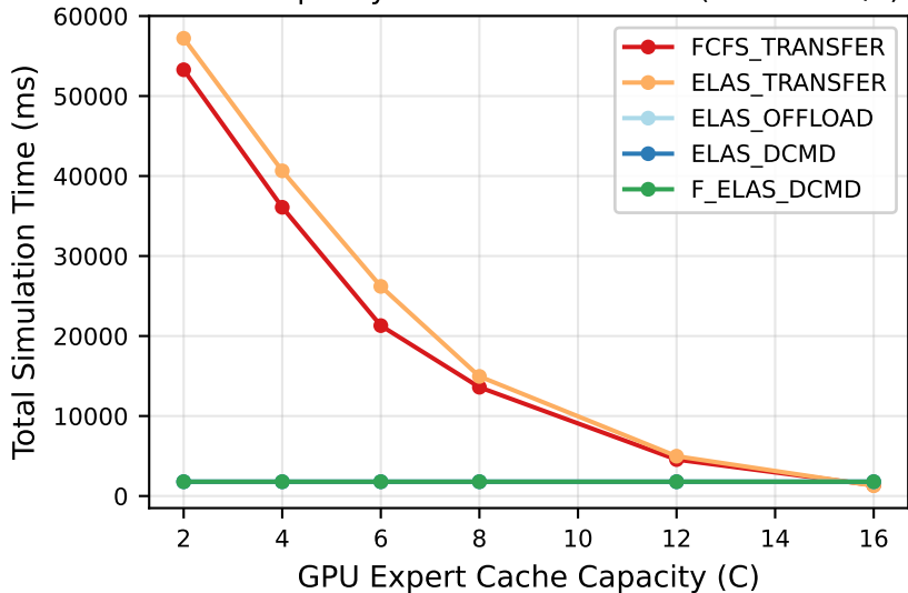
Cache Capacity vs. Simulation Time (BW=16GB/s)
