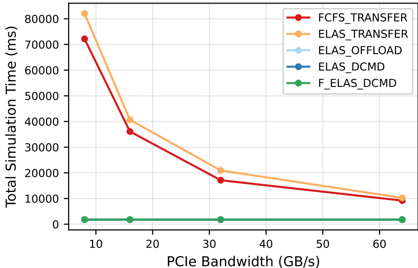
PCIe Bandwidth vs. Simulation Time (C=4)
