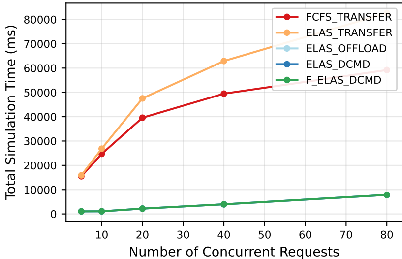
Concurrency Scaling (C=4, BW=16GB/s)
