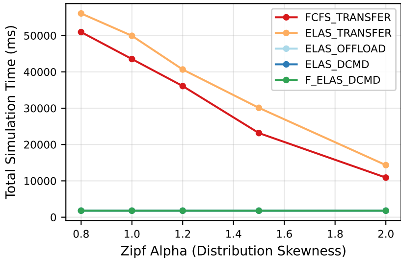
Workload Skewness Sensitivity (C=4, BW=16GB/s)
