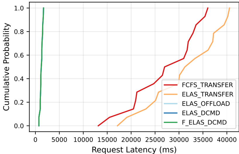
CDF of Request Latency (C=4, BW=16GB/s)
