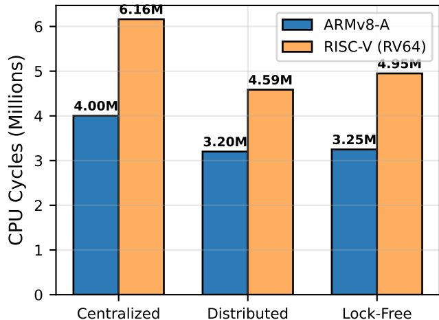
CPU Cycles Comparison
