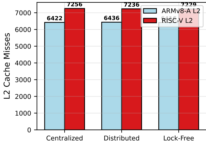
L2 Cache Performance
