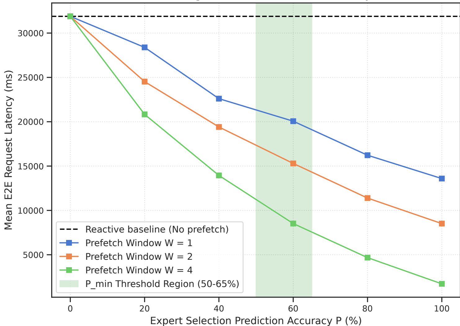
Prefetching Benefit vs. Prediction Accuracy
