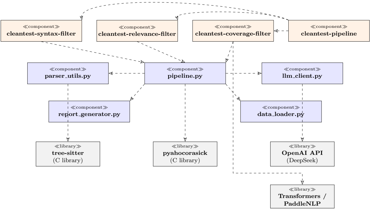
Fig. 5. Component Diagram: Module Dependencies
