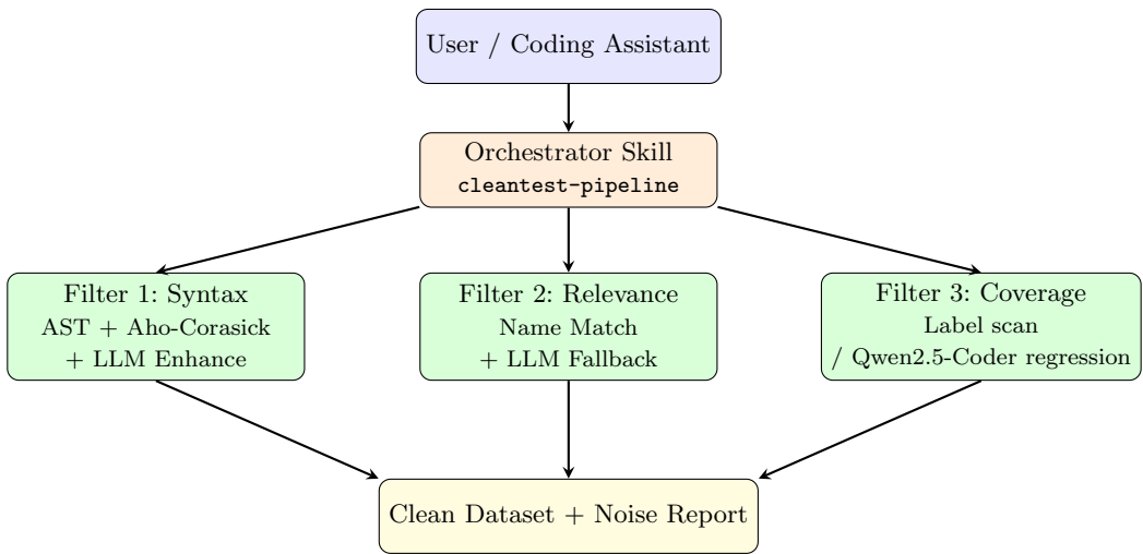
Fig. 4. CleanTest-Agent System Architecture
