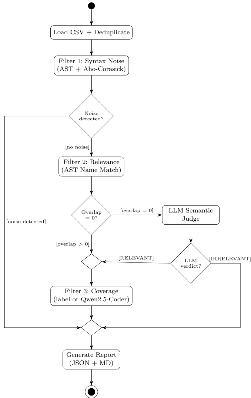
Fig. 2. Activity Diagram: Batch Cleaning Pipeline (UC1)
