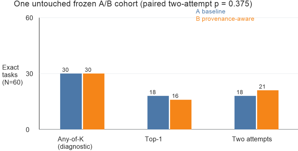
Figure 3: One untouched frozen A/B study (N=60). Any-of-K is diagnostic; two-attempt selection was fixed before target scoring.
