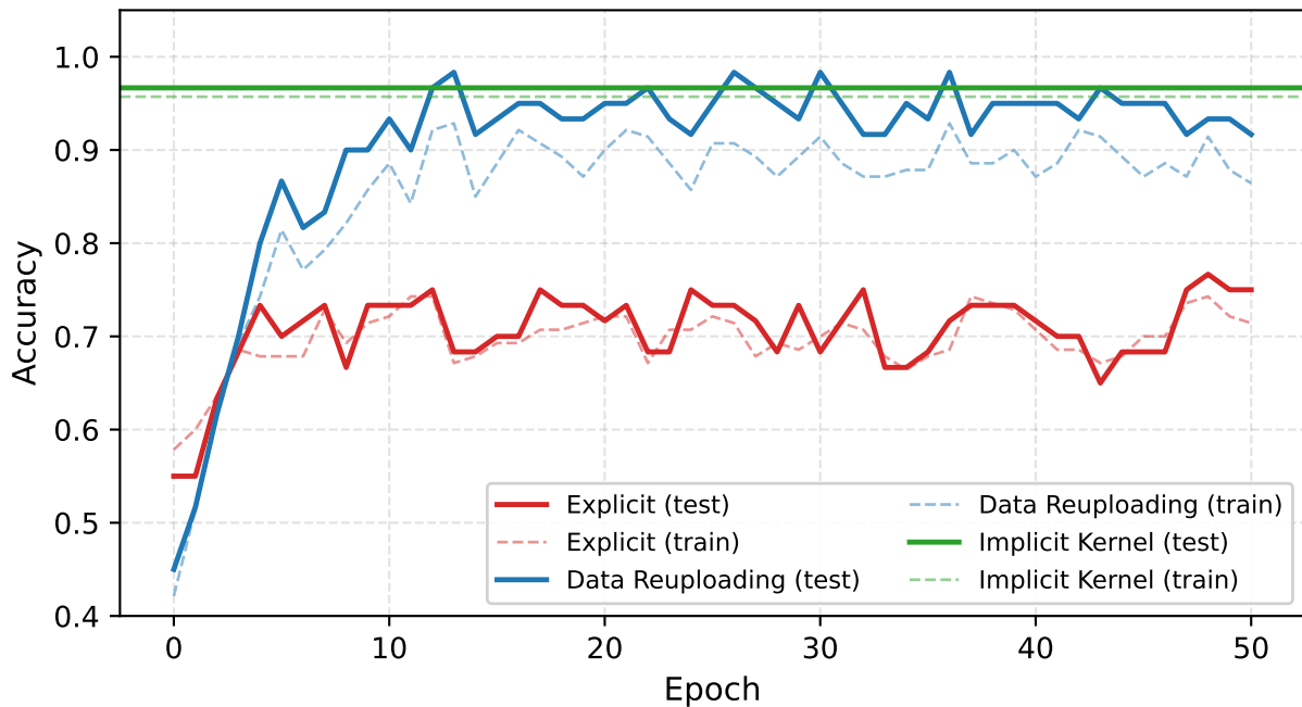
Problem 2 (a) — Circle Dataset: Accuracy vs Epoch (reproducing Ref. [3] Fig. 6)
