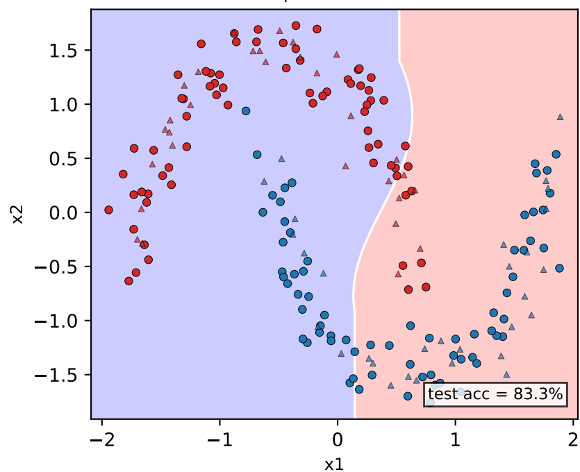
Implicit Kernel - moons
