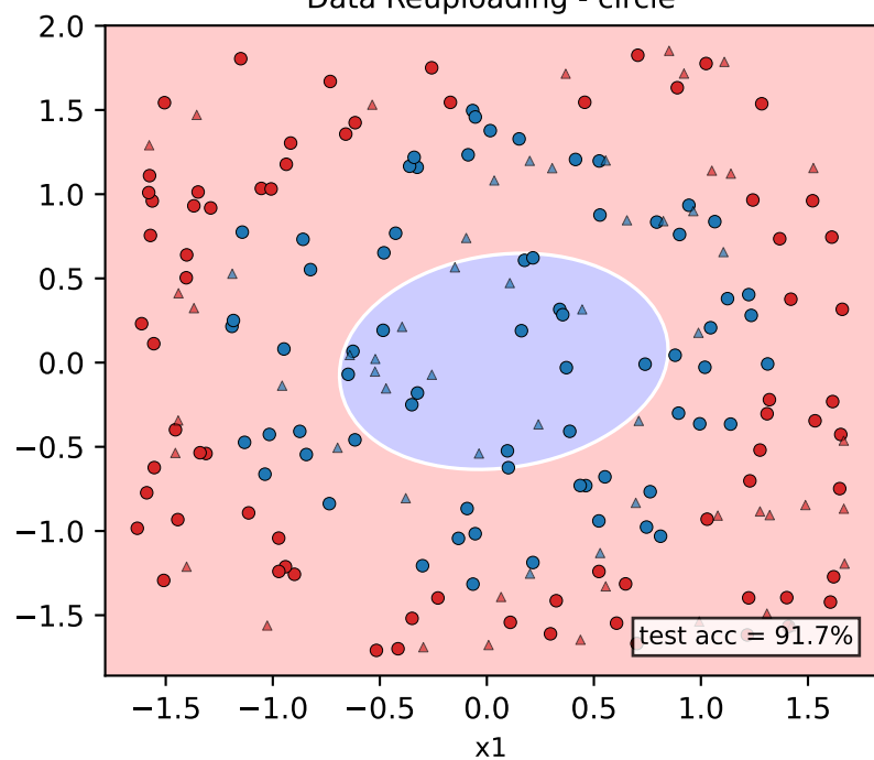
Data Reuploading - circle
