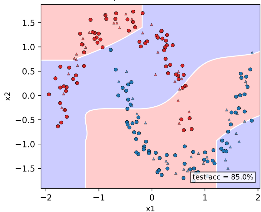
Data Reuploading - moons
