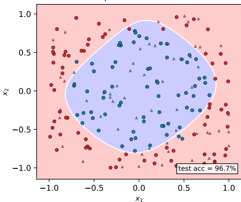
Data Reuploading — circle
