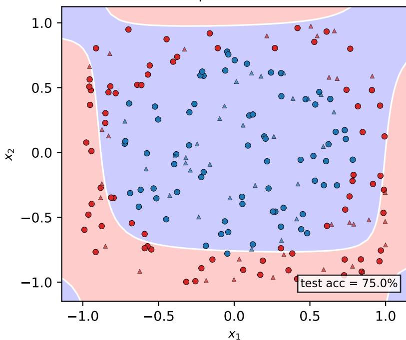
Implicit Kernel — circle
