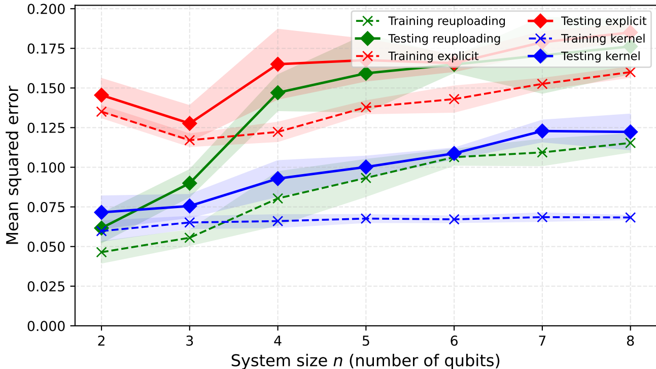
Regression performance on hypersphere dataset (reproducing Ref. [3] Fig. 6, n = system size)
