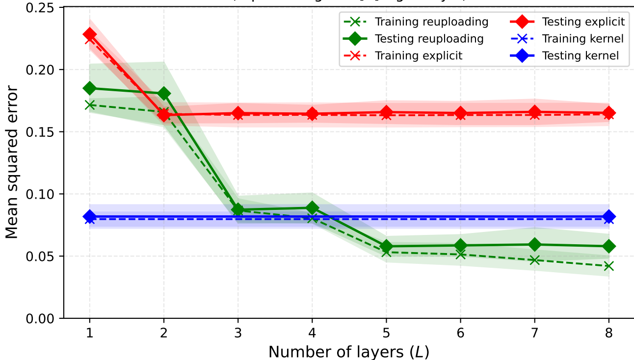
Regression performance on circle dataset (reproducing Ref. [3] Fig. 6 style)
