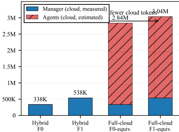
Cloud tokens per 10-gen run
