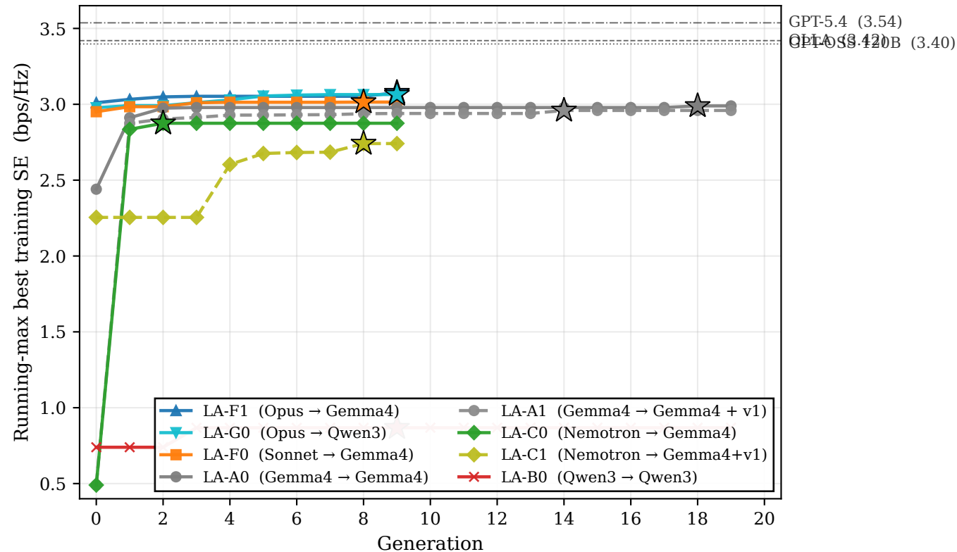
Running-max best score per generation, all configurations ( * marks the generation in which each run's all-time best was first achieved)
