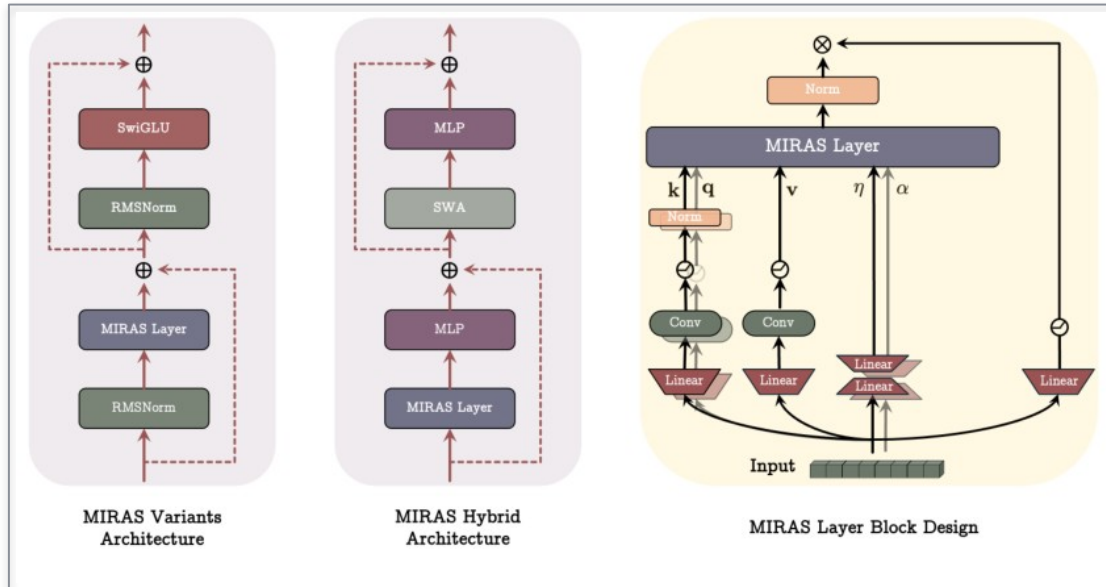
Figure 2 — Moneta/Yaad/Memora: recurrent · SWA hybrid · layer 설계
