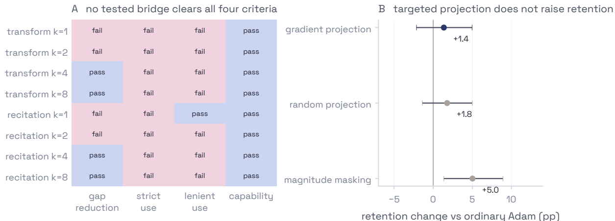
Figure 18: Intervention controls. A: Each row is an eligible tested 144-step bare-statement plus 48-step bridge condition; indigo marks a passed individual criterion. No row passes all four. B: Retention change relative to ordinary Adam. Targeted gradient projection gains 1.4 points, random projection 1.8, and magnitude masking 5.0. Intervals resample the 60 paired store–seed–fact units; only five stored facts are unique.
