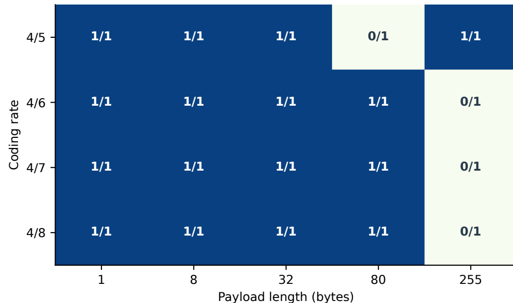
A SF7: full packet CRC + exact bytes
