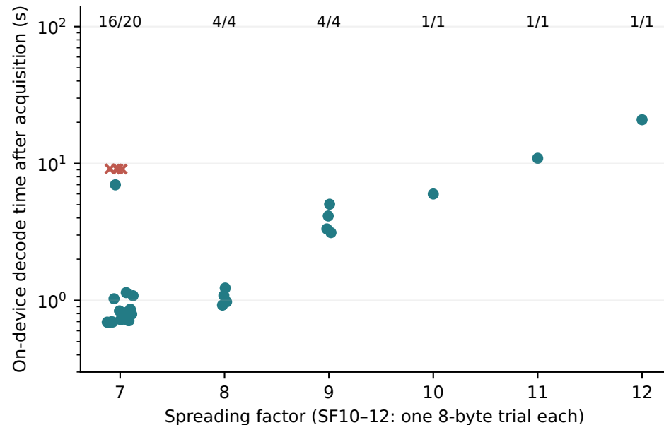
B Native latency and accepted/attempted counts
