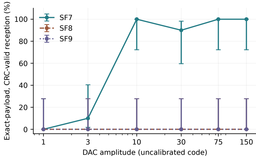
A Amplitude sweep, 10 trials per point
